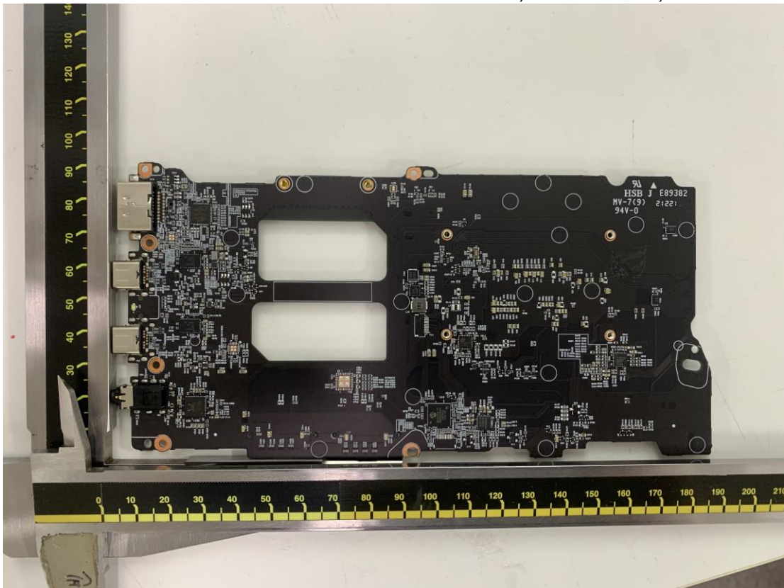
Figure 37 1xZ90P MAIN B/D PCB, Main Board, Front View
