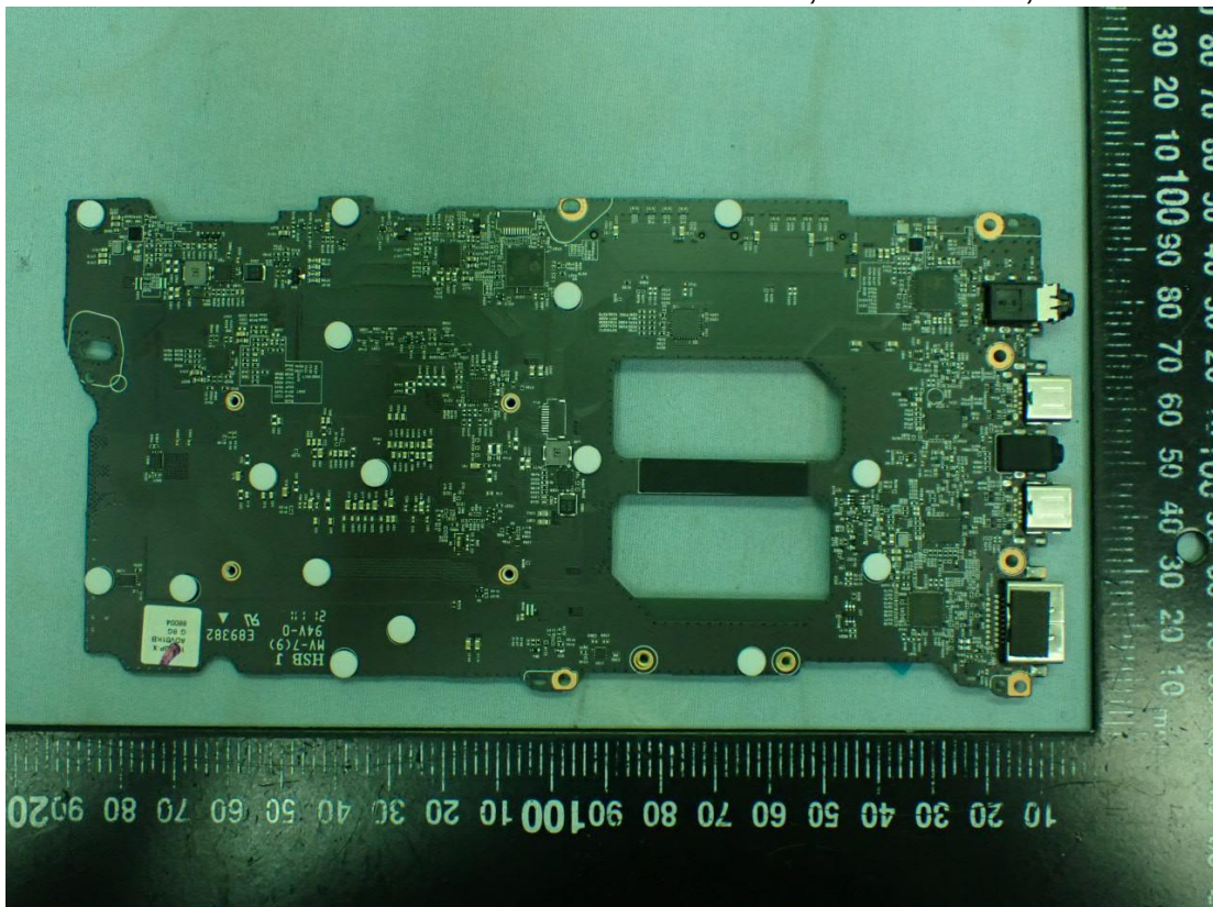
Figure 36 Blanc MAIN B/D PCB, Main Board, Back View
