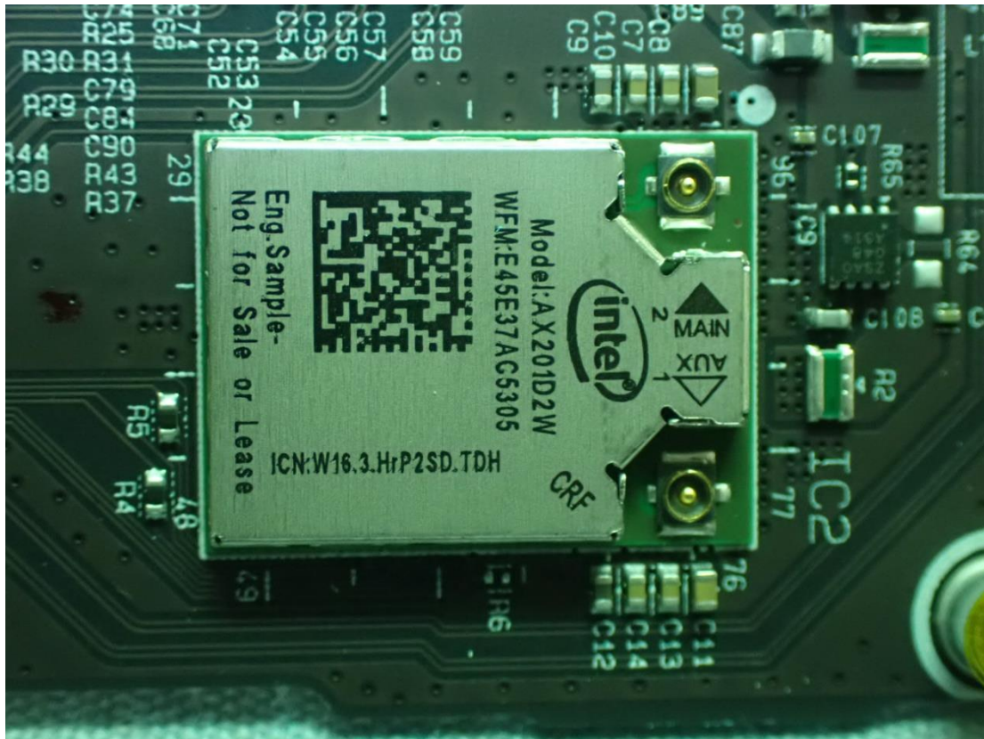
Figure 51 WLAN Combo Card View
