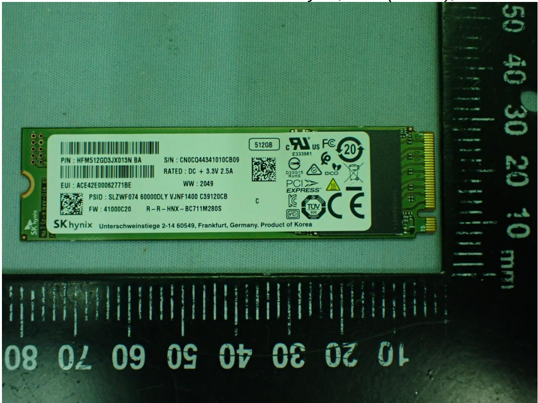
Figure 45 SK hynix, SSD (512GB), Front View
