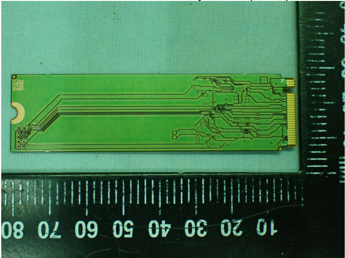
Figure 46 SK hynix, SSD (512GB), Back View
