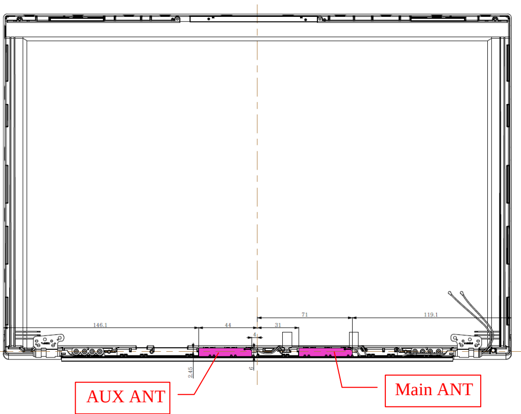
Figure 55 Antenna Position
