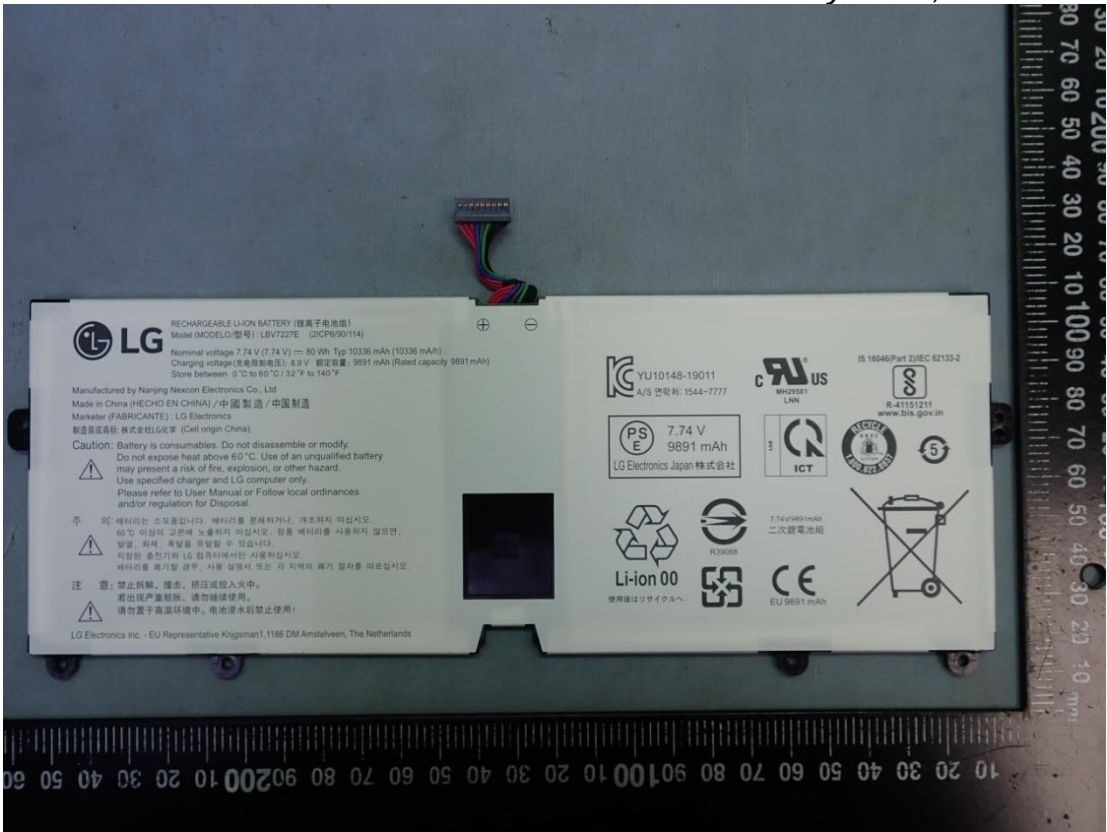
Figure 42 Battery Pack, Back View
