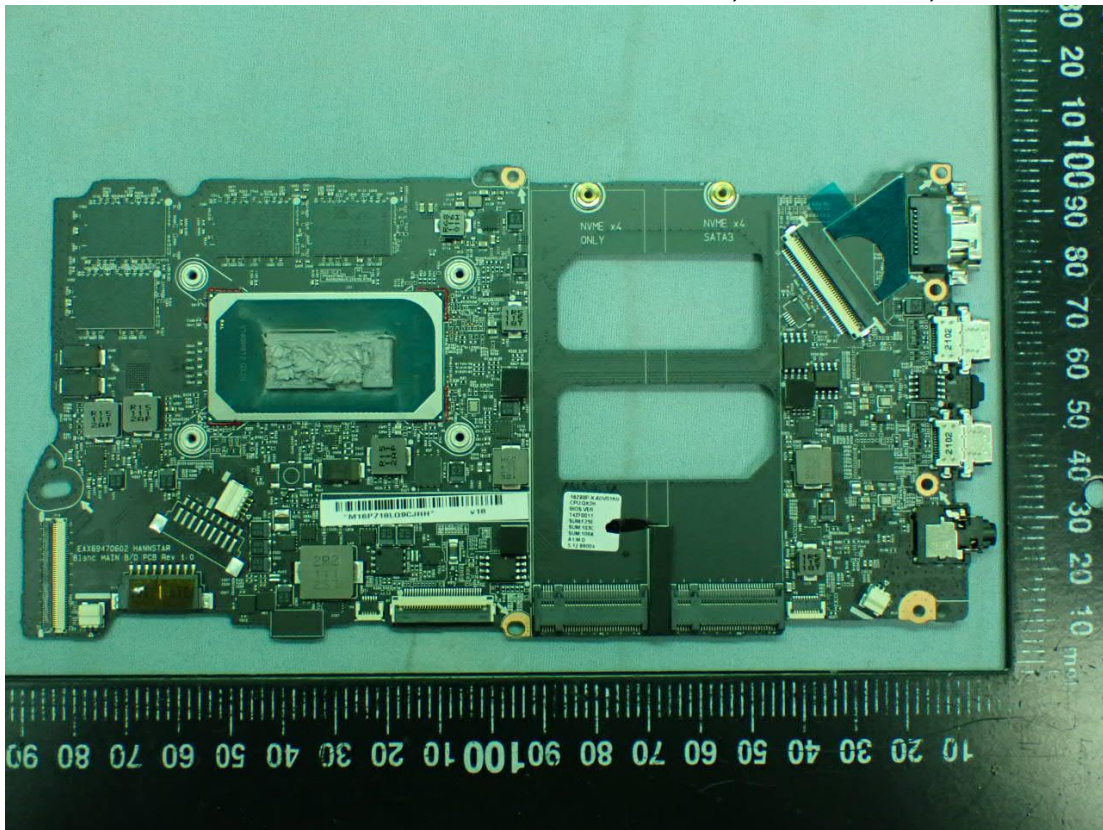
Figure 35 Blanc MAIN B/D PCB, Main Board, Front View
