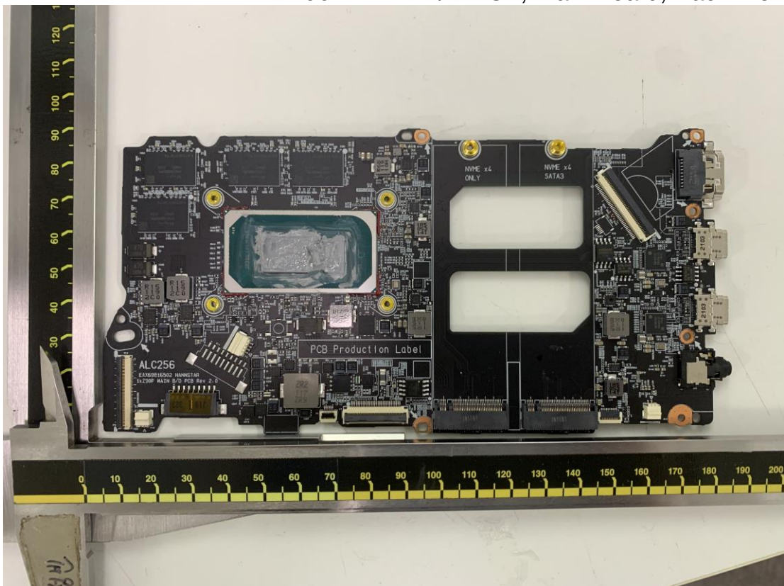
Figure 38 1xZ90P MAIN B/D PCB, Main Board, Back View
