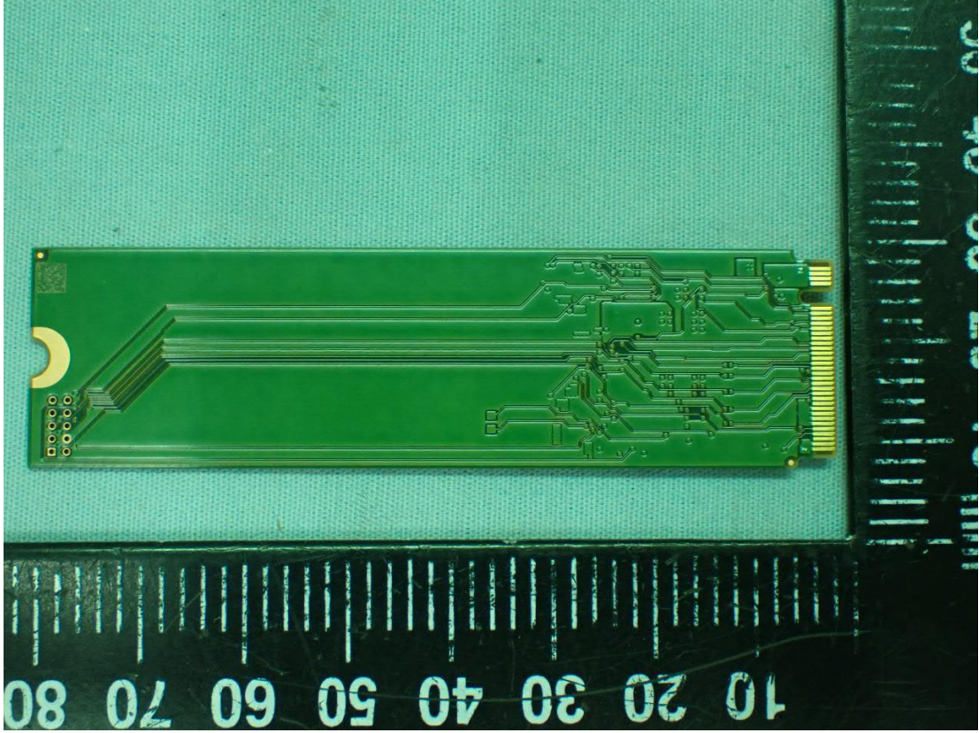
Figure 44 SK hynix, SSD (256GB), Back View
