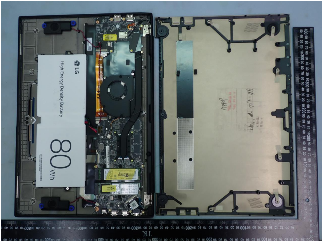
Figure 34 Internal View
