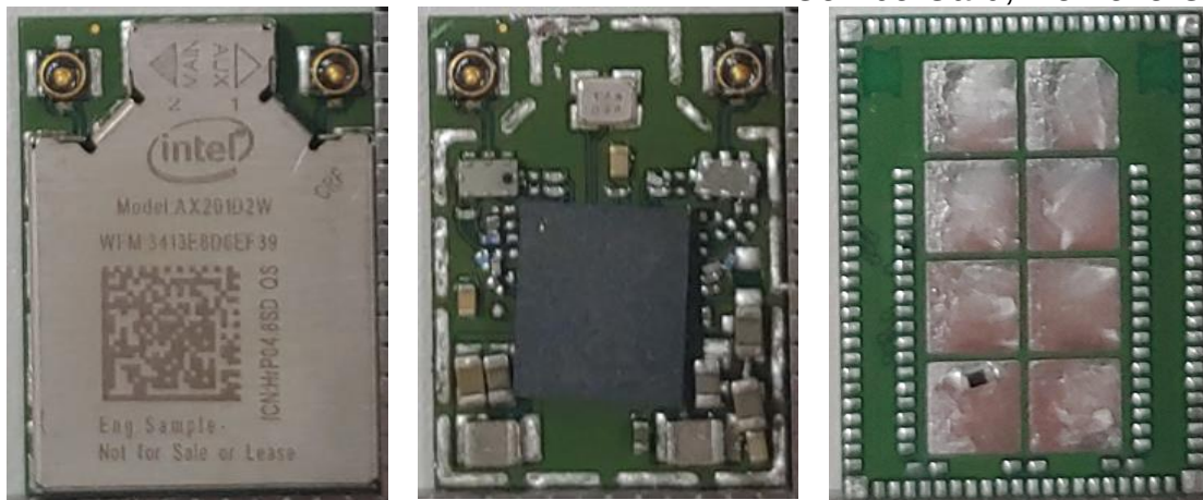
Figure 52 WLAN Combo Card, Remove Cover
