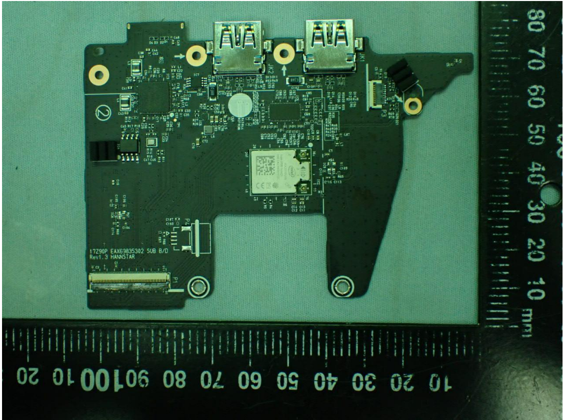
Figure 39 WLAN SUB Board, Front View
