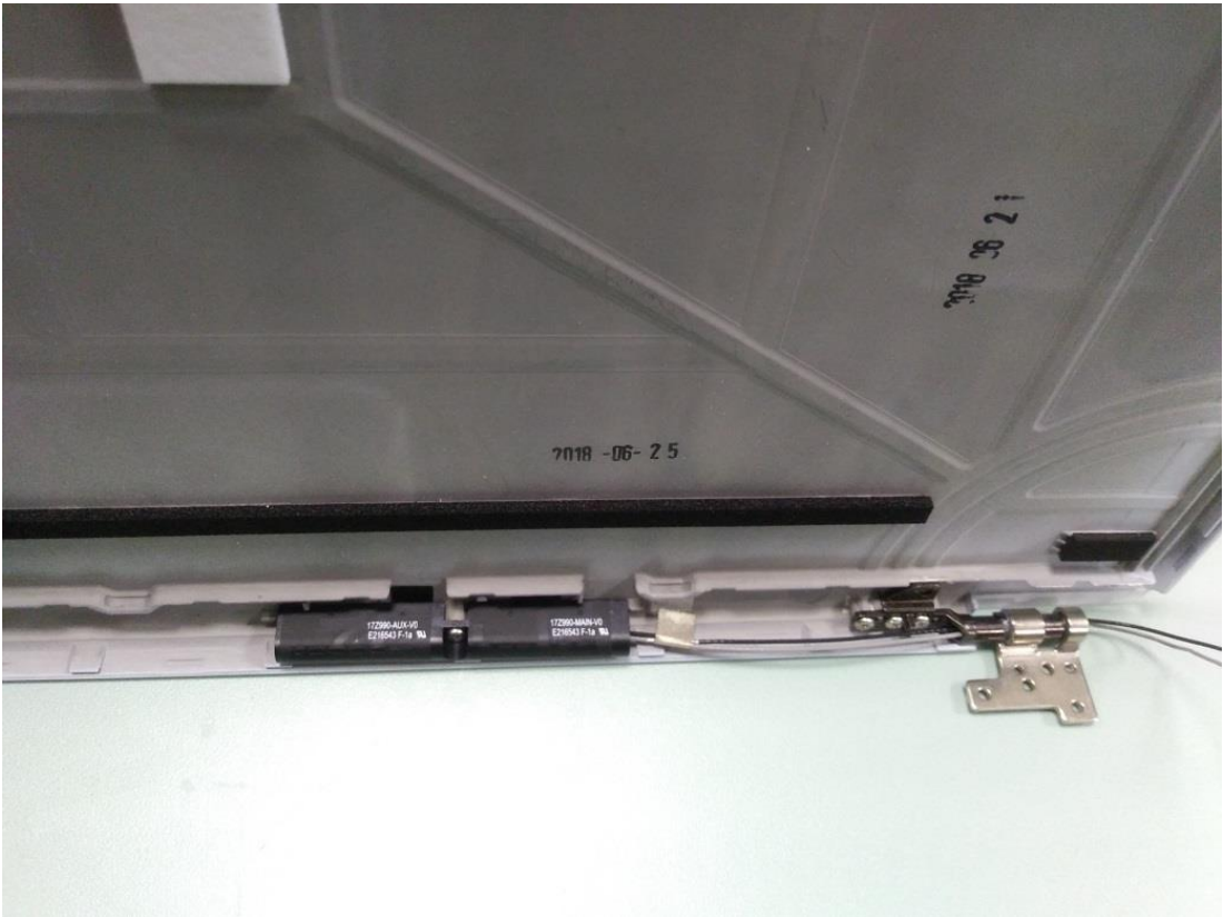
Figure 45 WLAN Antenna Position
