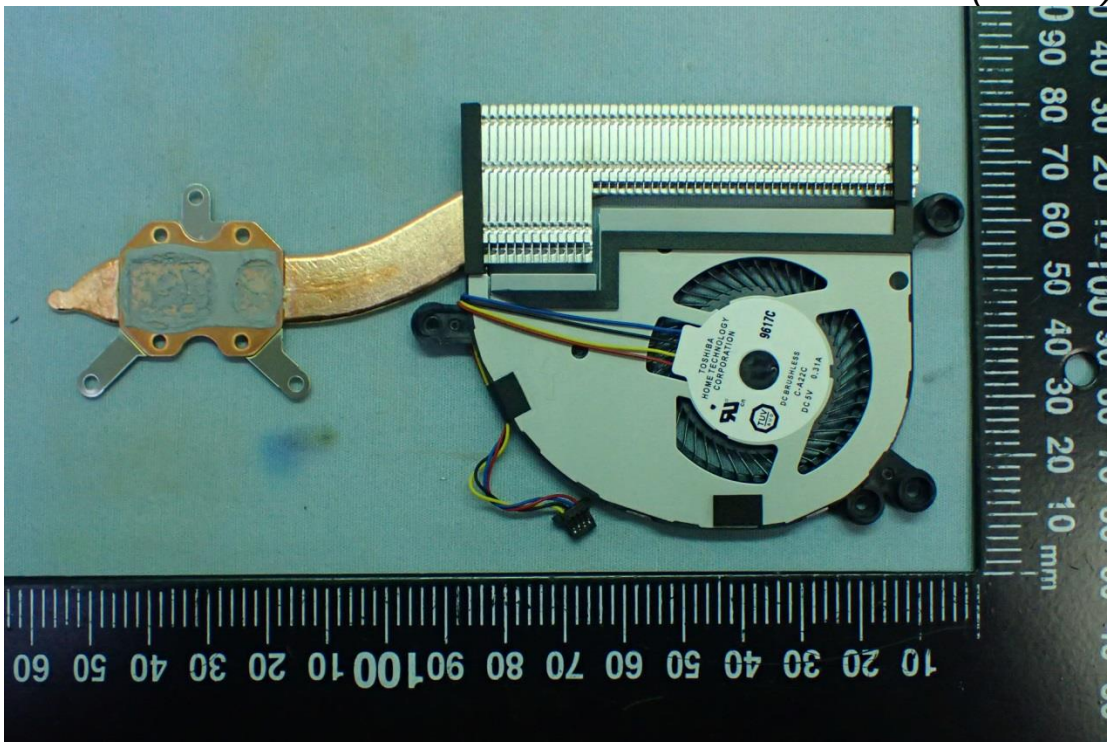
Figure 41 Internal View (DC Fan)
