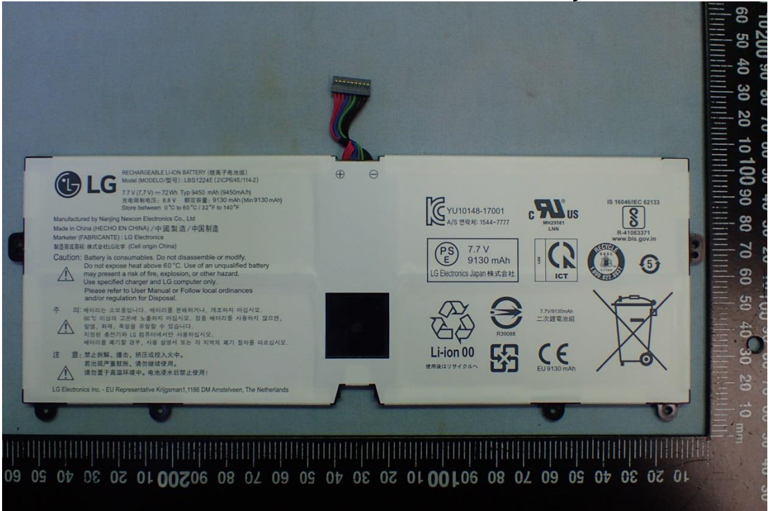
Figure 48 Battery Pack, Back View
