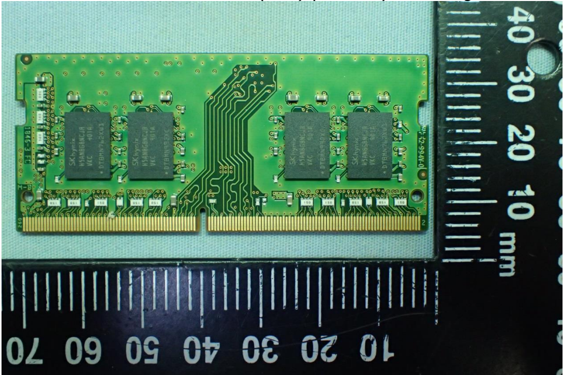
Figure 52 RAM (8GB) (On Card), Samsung, Back View
