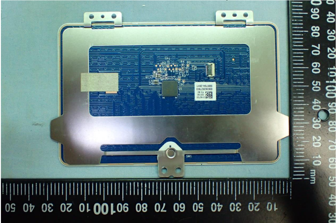
Figure 29 Internal View (Touch Pad, Back View)
