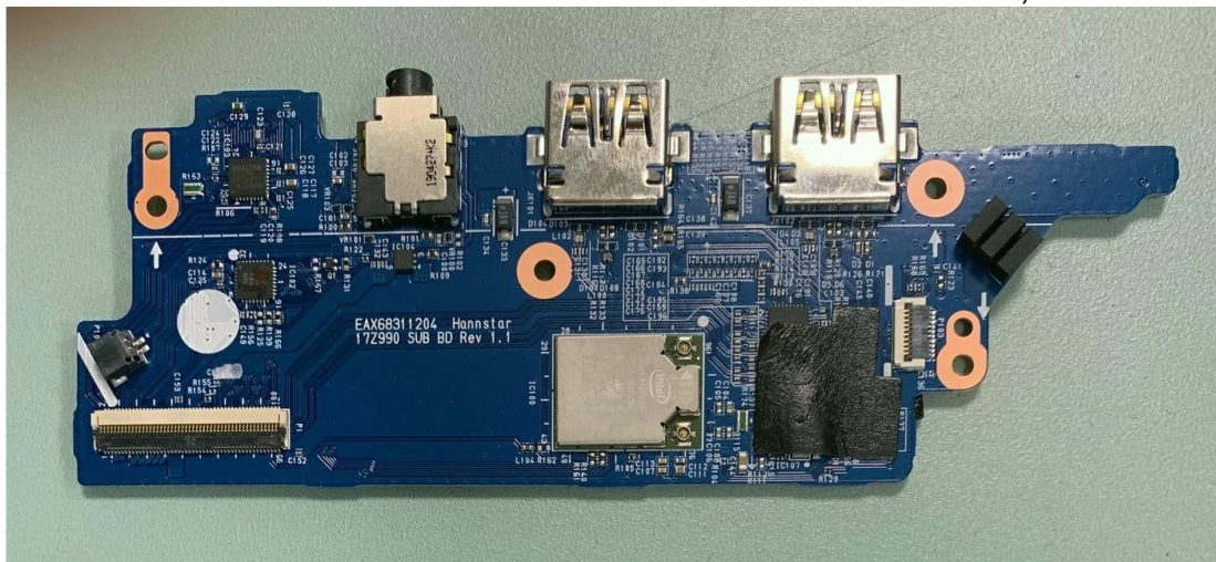
Figure 37 SUB Board, Front View
