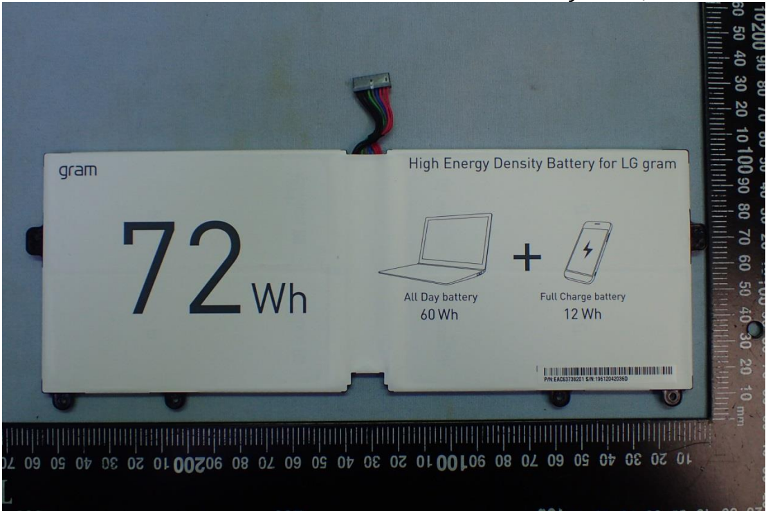
Figure 47 Battery Pack, Front View
