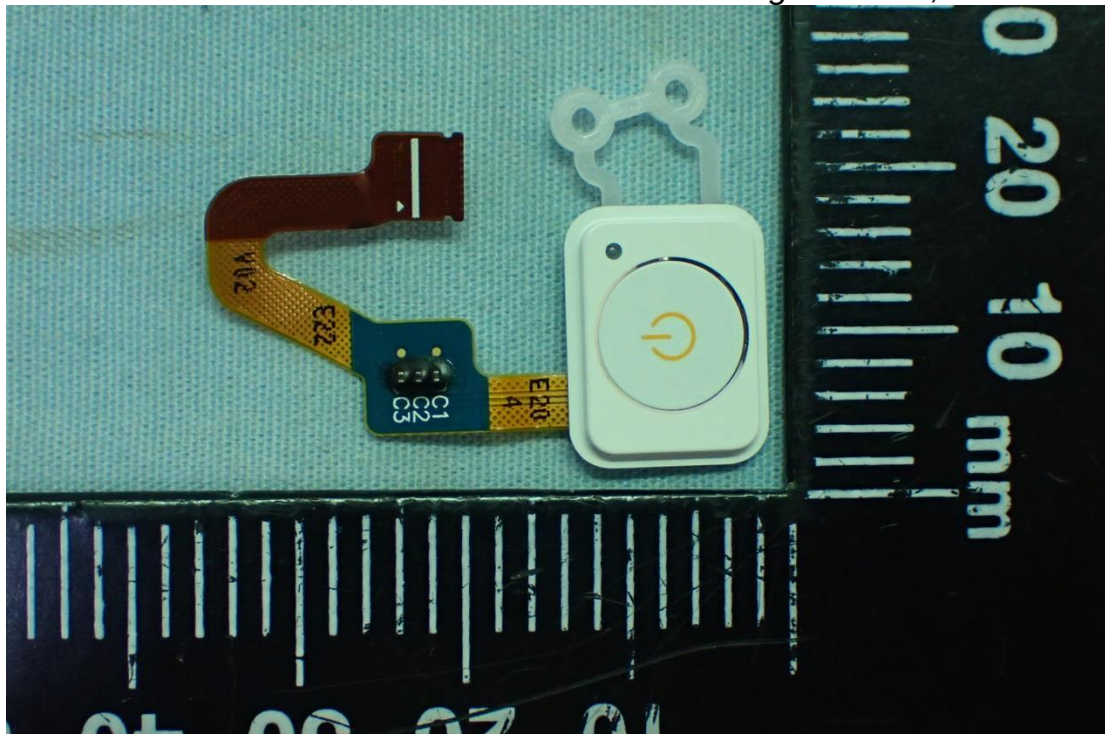
Figure 35 Finger Printer, Front View
