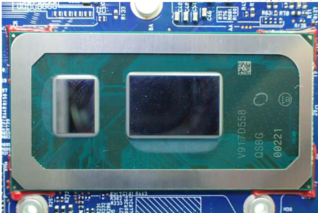
Figure 34 i5-10210U, CPU View
