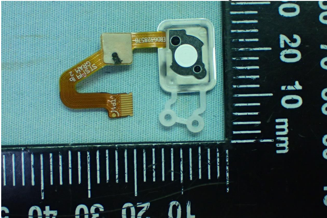
Figure 36 Finger Printer, Back View
