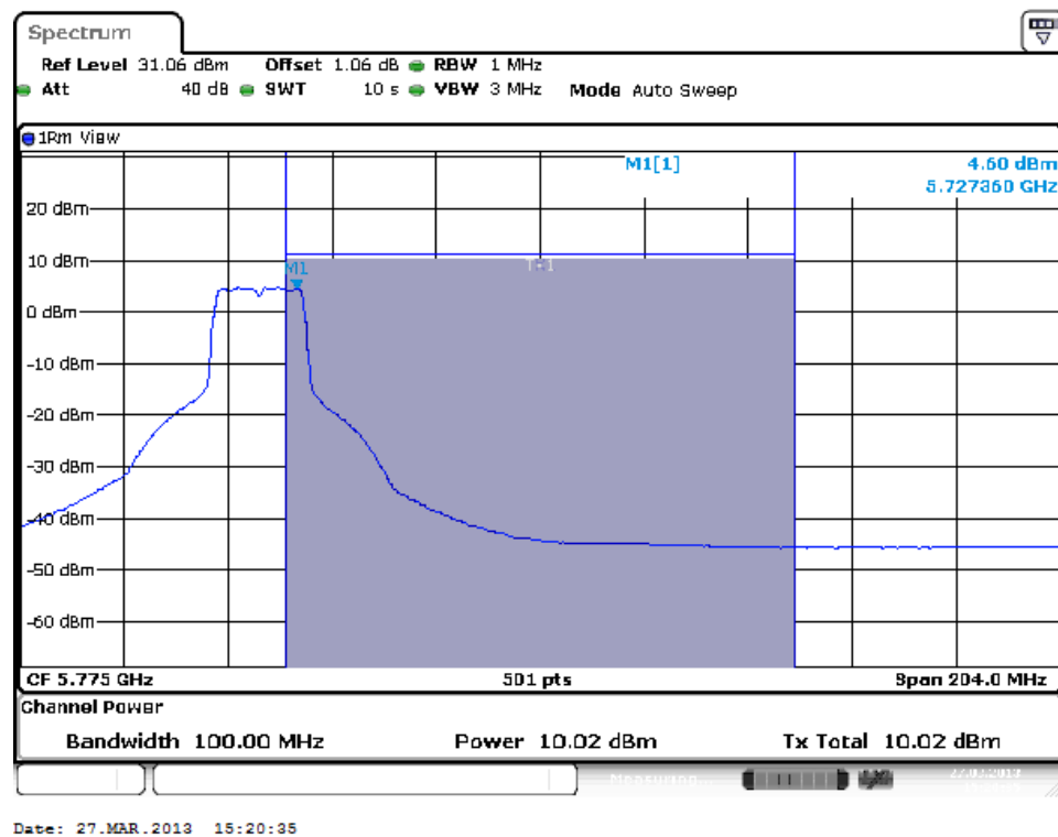
Power and PPSD in UNII 3
