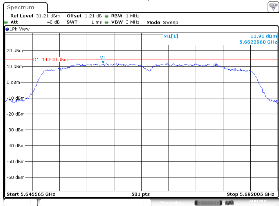
Plot Antenna 1, 5670 MHz
