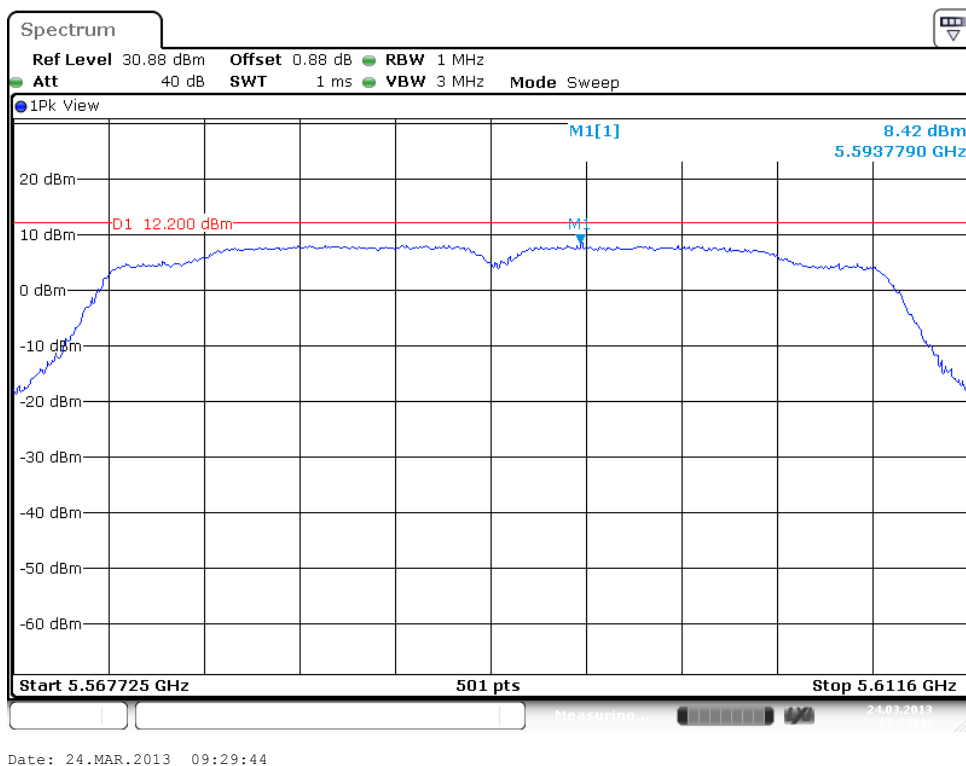
Plot Antenna 2 , 5590 MHz
