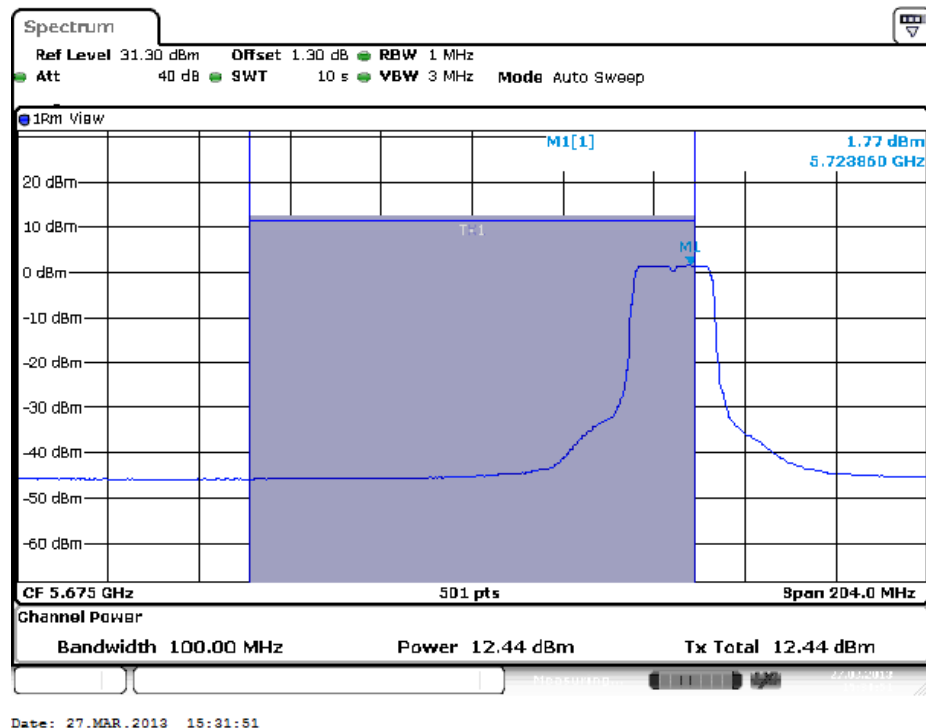
Power and PPSD in UNII 2ext, Antenna 1
