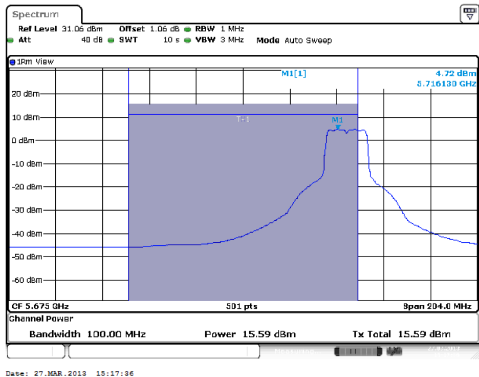
Power and PPSD in UNII 2ext
