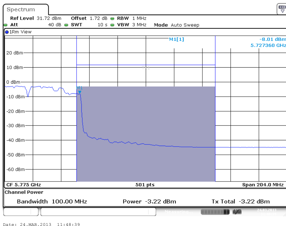
Plot VHT6 80 MHz, Antenna 2 U-NII 3
