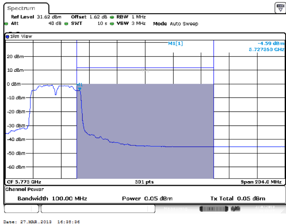
Power and PPSD in UNII 3, Antenna 1
