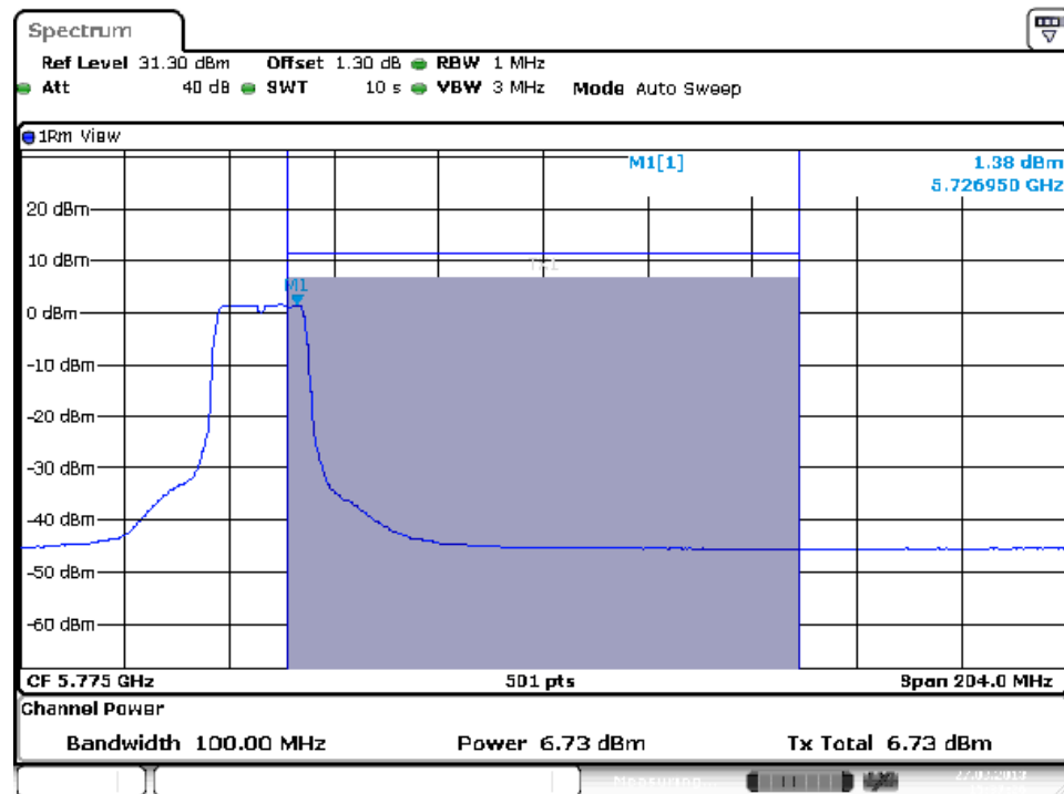
Power and PPSD in UNII 3, Antenna 1
