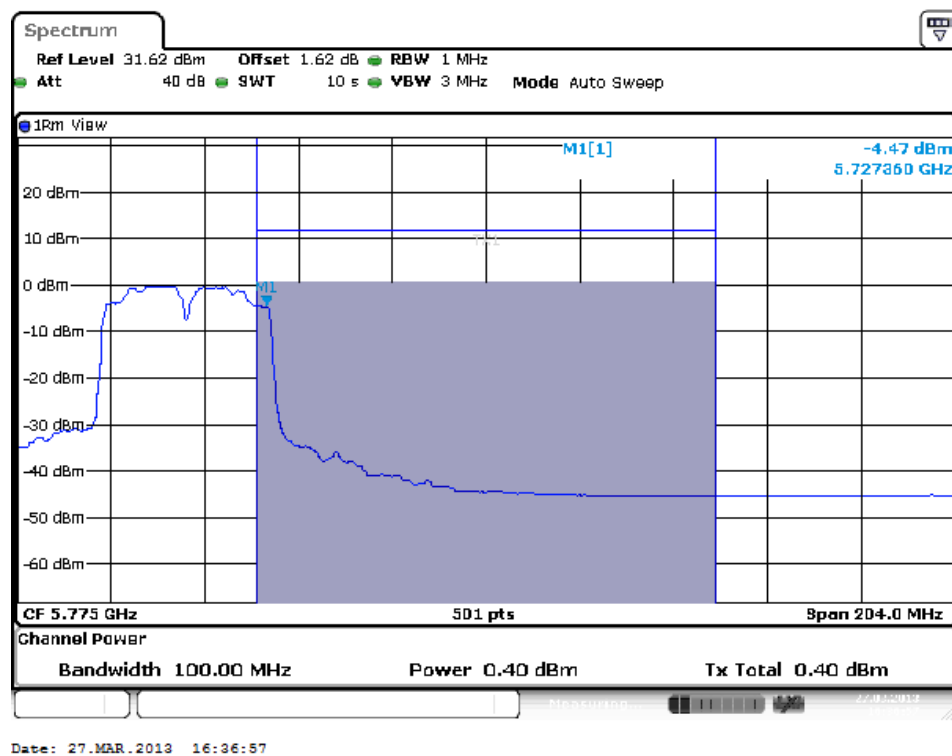
Power and PPSD in UNII 3, Antenna 2
