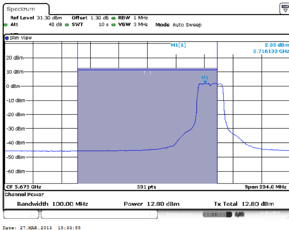
Power and PPSD in UNII 2ext, Antenna 2
