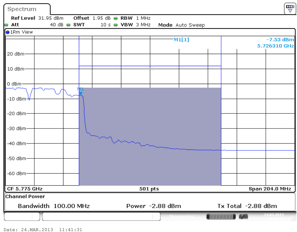
Plot B2 Antenna2 at 5690 MHz UNII 3 band
