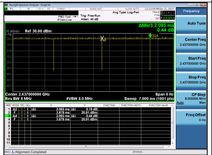
Duty cycle data : TM 2 & 6 Mbps & Middle
