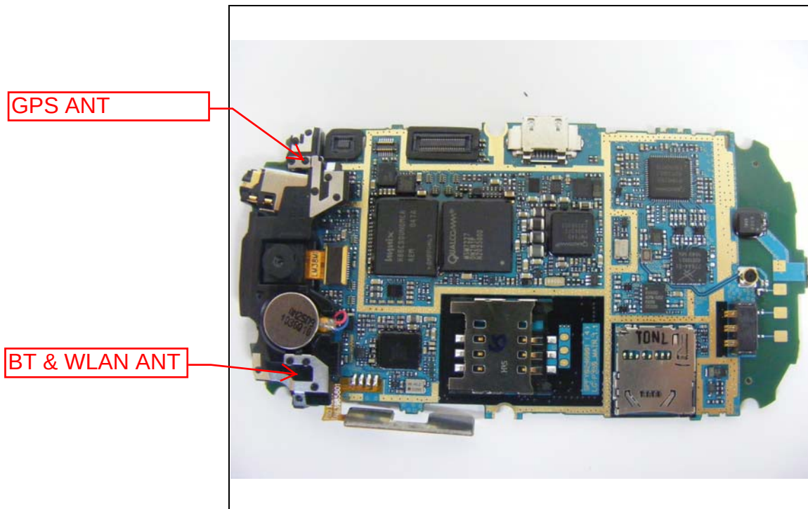
Bottom view of main board
