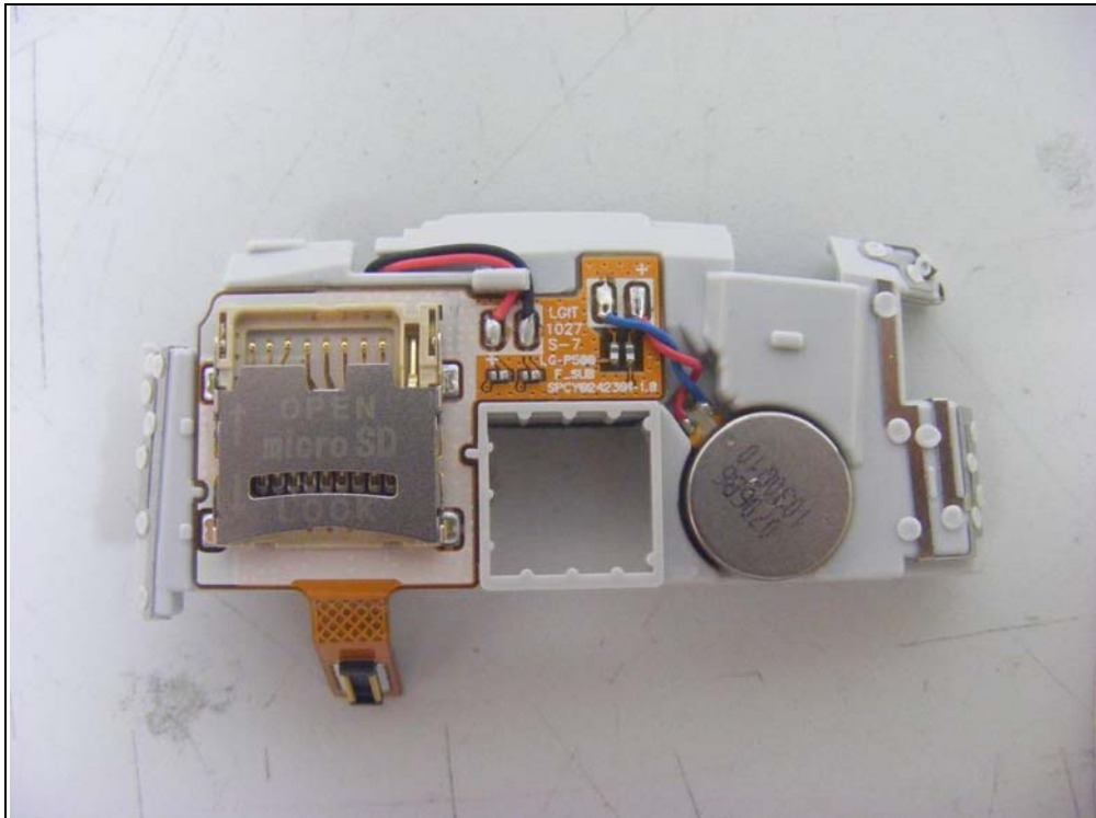
Bottom view of Sub Board
