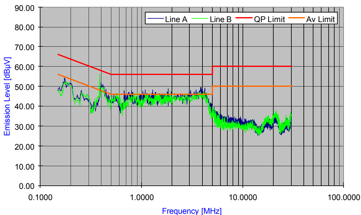
Plot 6-18. Line Conducted Plot with 802.11g
