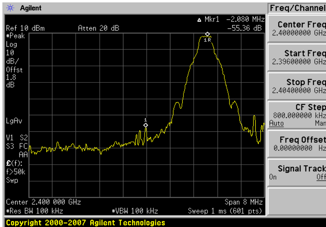
Plot 6-10. Band Edge Plot (Bluetooth, 1Mbps – Ch. 0)
