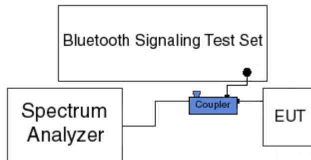
Figure 6-2. Test Instrument & Measurement Setup
