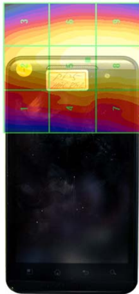
Figure 17-4 E-Field WD Scan overlay
