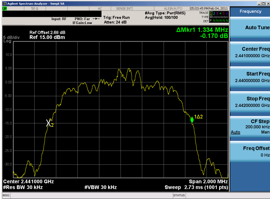
Plot 6-5. 20dB Bandwidth Plot (Bluetooth, 2Mbps – Ch. 39)
