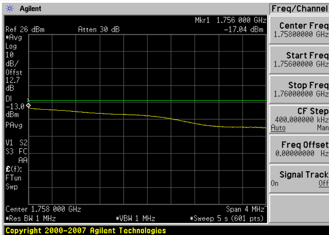
Plot 7-45. 4MHz Span Plot (AWS WCDMA Mode – Ch. 1862)
