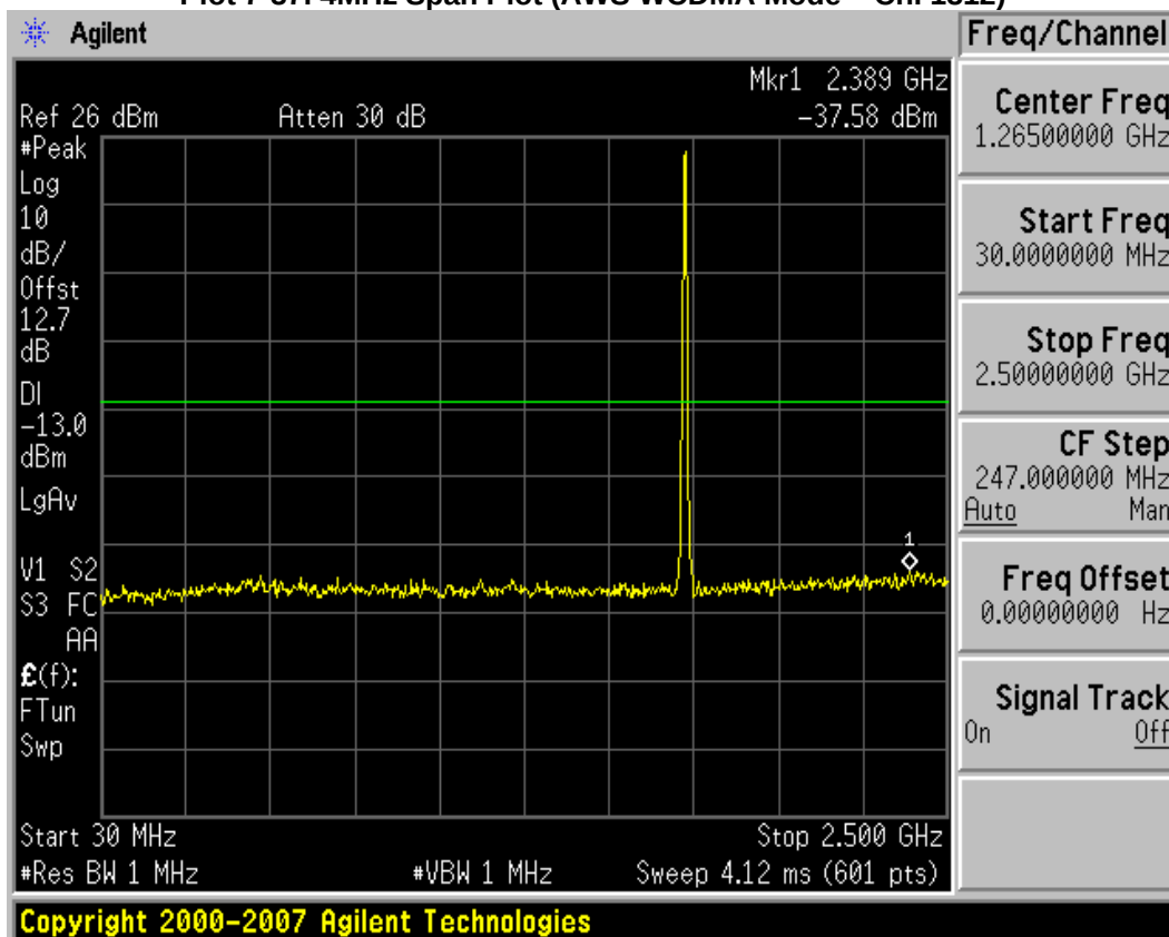
Plot 7-38. Conducted Spurious Plot (AWS WCDMA Mode – Ch. 1412)
