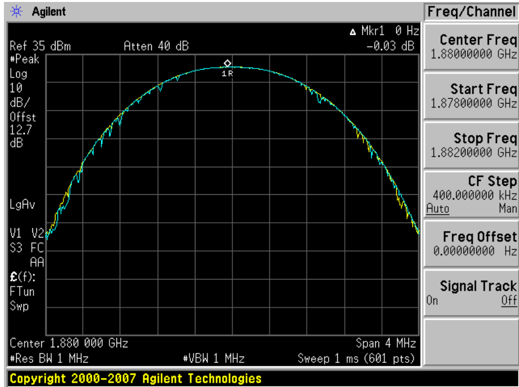
Plot 7-33. Peak-Average Ratio Plot (EDGE1900 Mode – Ch. 661)
