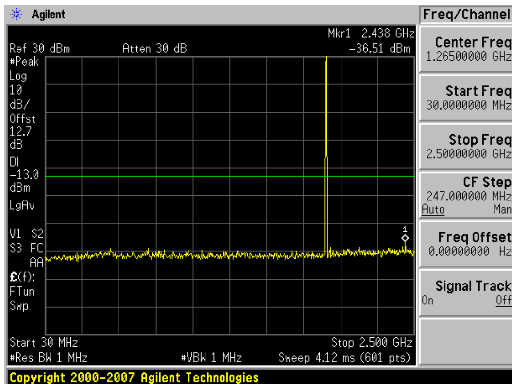
Plot 7-29. Conducted Spurious Plot (PCS GSM Mode – Ch. 810)
