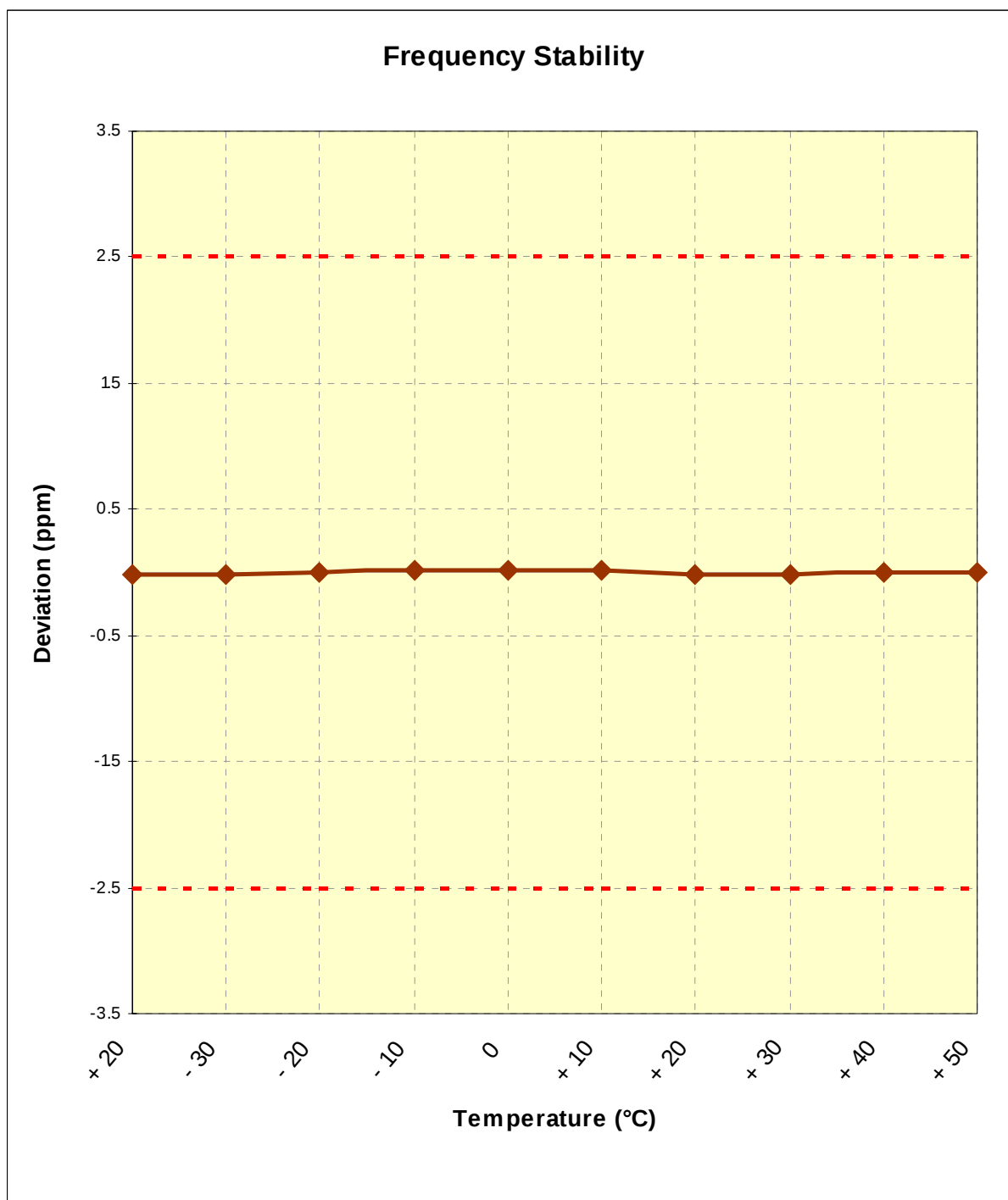
Figure 6-4. Frequency Stability Graph (AWS WCDMA Mode – Ch. 1412)
