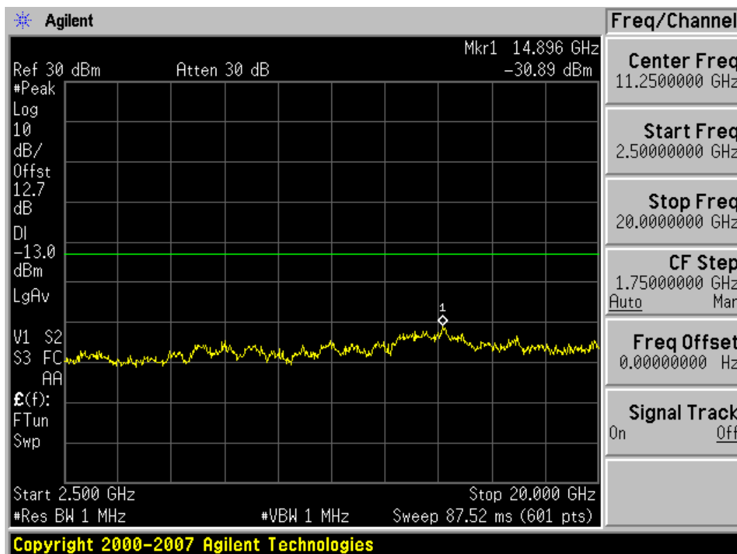
Plot 7-23. Conducted Spurious Plot (PCS GSM Mode – Ch. 512)
