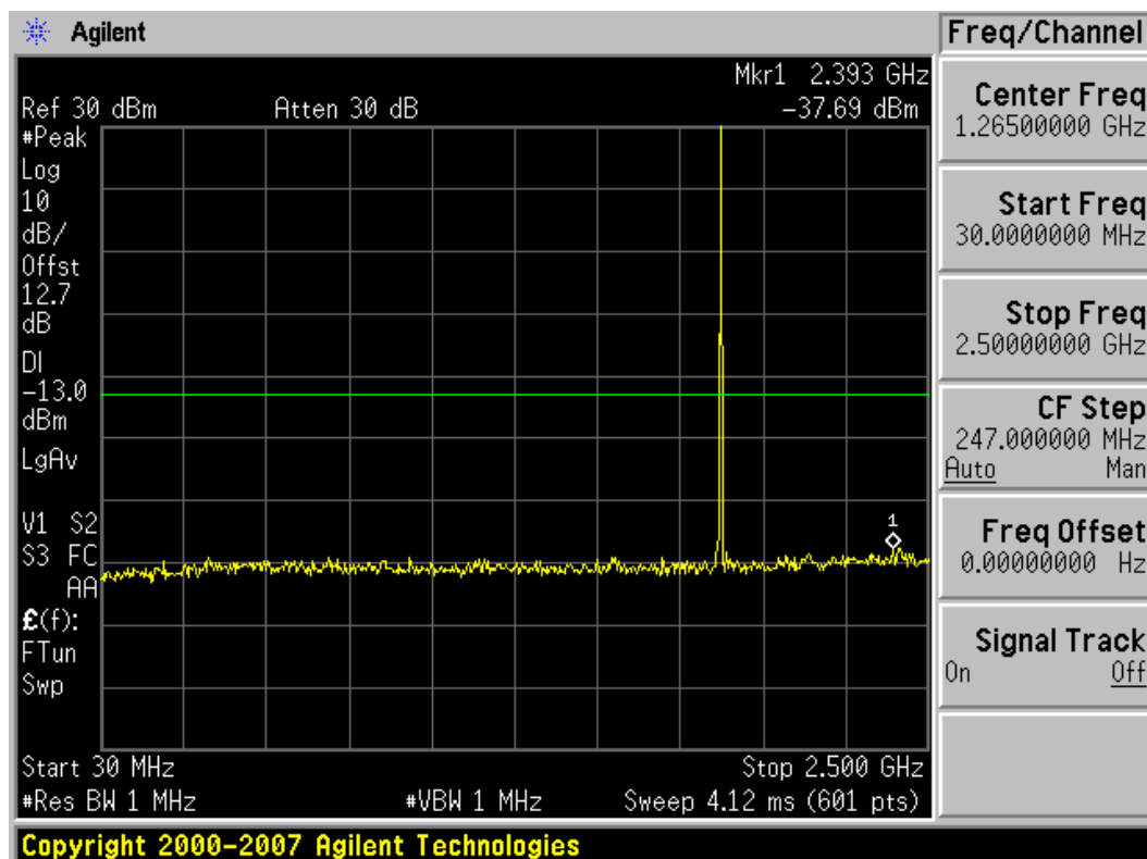
Plot 7-25. Conducted Spurious Plot (PCS GSM Mode – Ch. 661)
