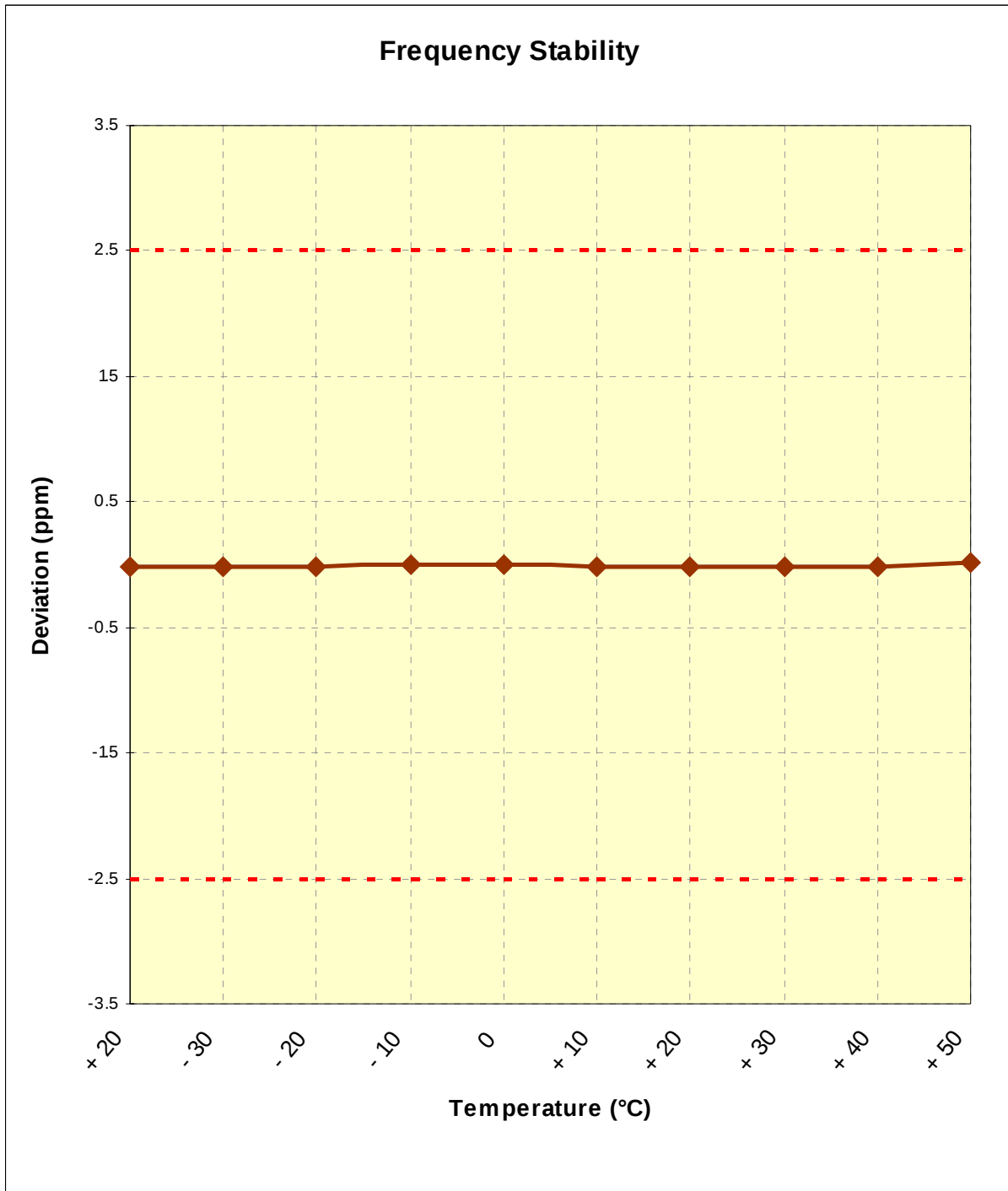
Figure 6-3. Frequency Stability Graph (PCS GSM Mode – Ch. 661)
