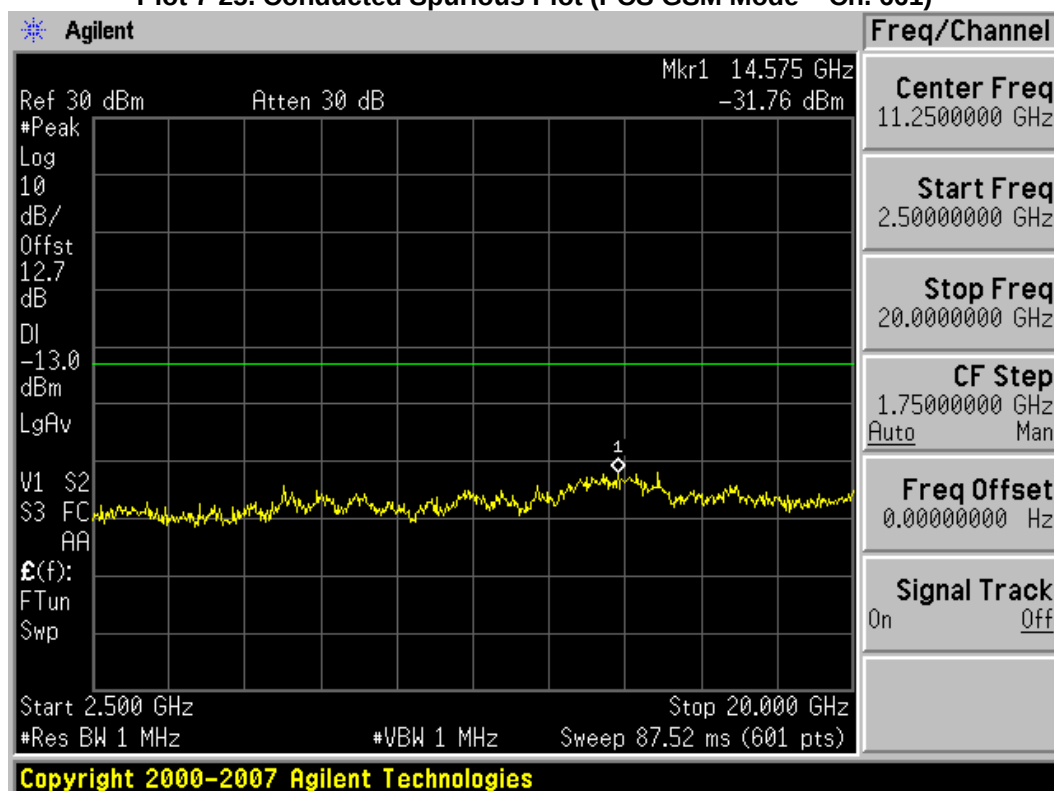
Plot 7-26. Conducted Spurious Plot (PCS GSM Mode – Ch. 661)
