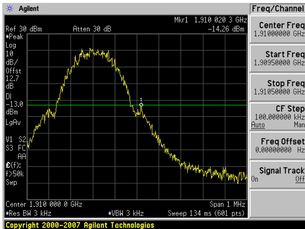
Plot 7-31. Band Edge Plot (PCS GSM Mode – Ch. 810)
