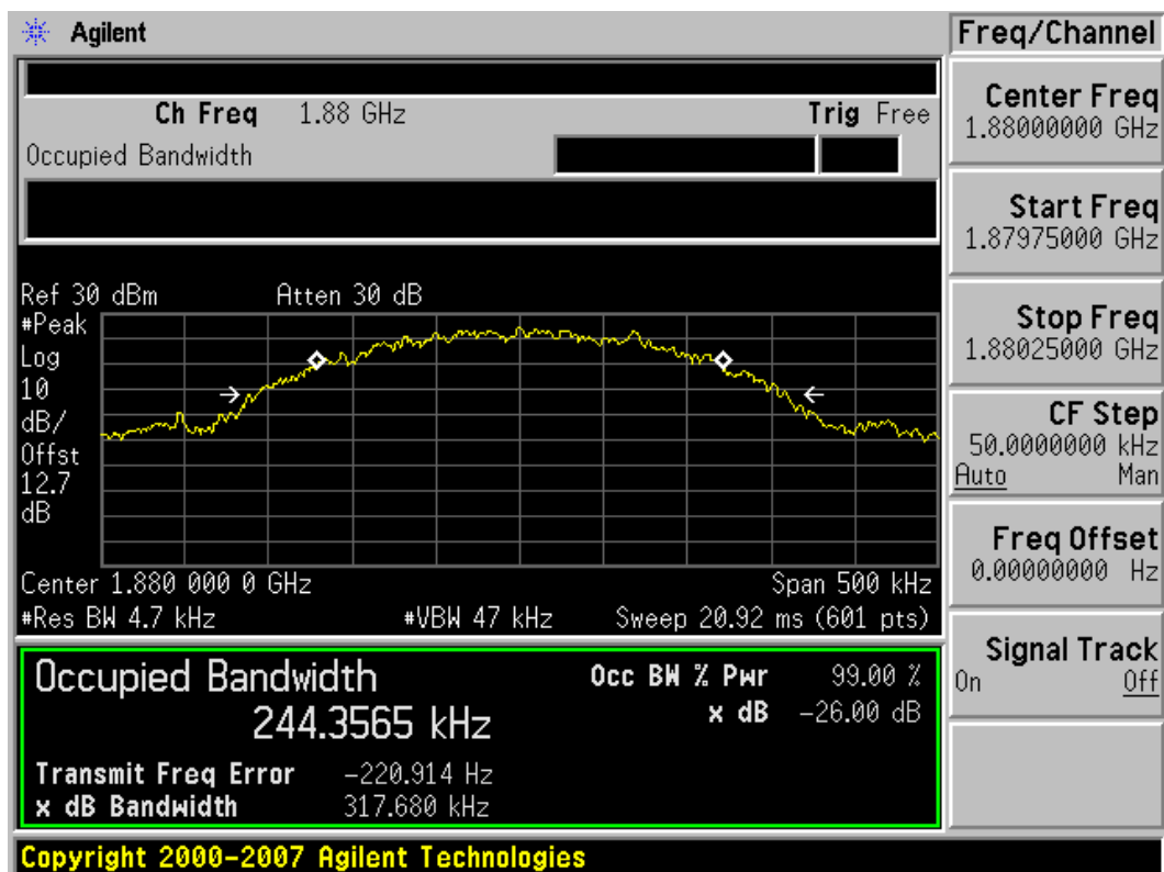
Plot 7-27. Occupied Bandwidth Plot (PCS GSM Mode – Ch. 661)
