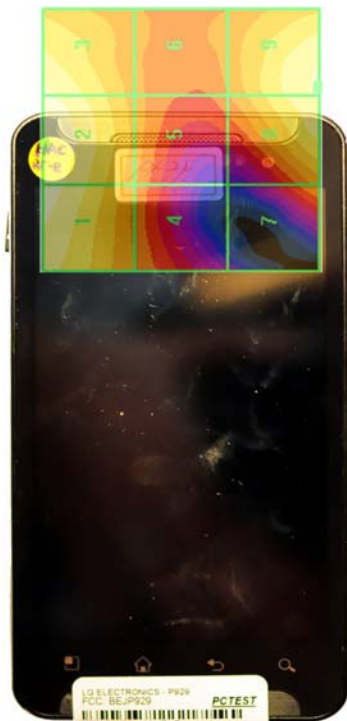
Figure 17-4 E-Field WD Scan overlay
