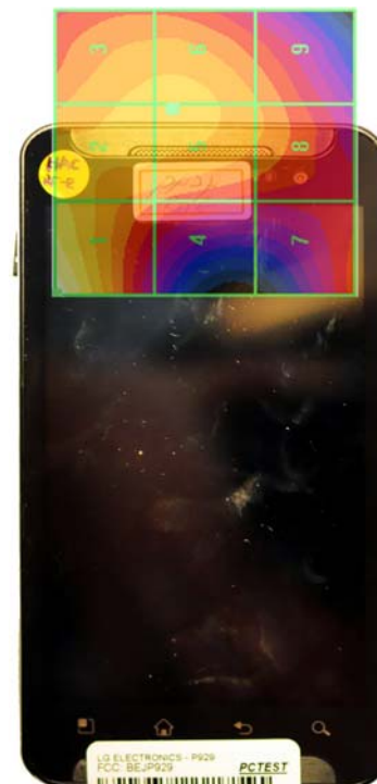
Figure 17-5 H-Field WD Scan overlay
