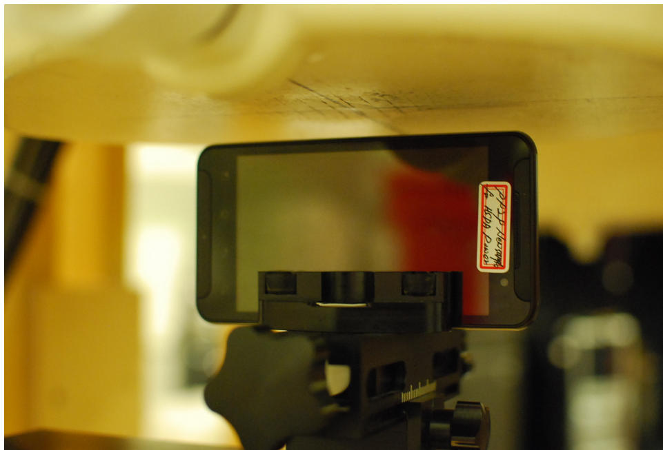
Figure 21-10 SAR Test Setup Photo 10 – Left at 1.0 cm
