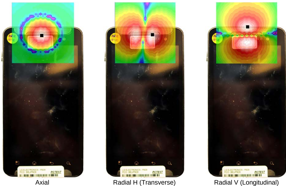
Figure 13-3 T-Coil Scan Overlay Magnetic Field Distributions
