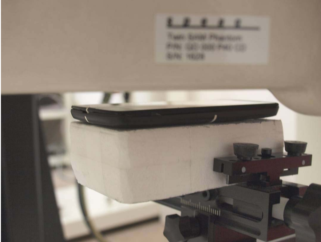
BODY – FRONT with 10 mm Separation
