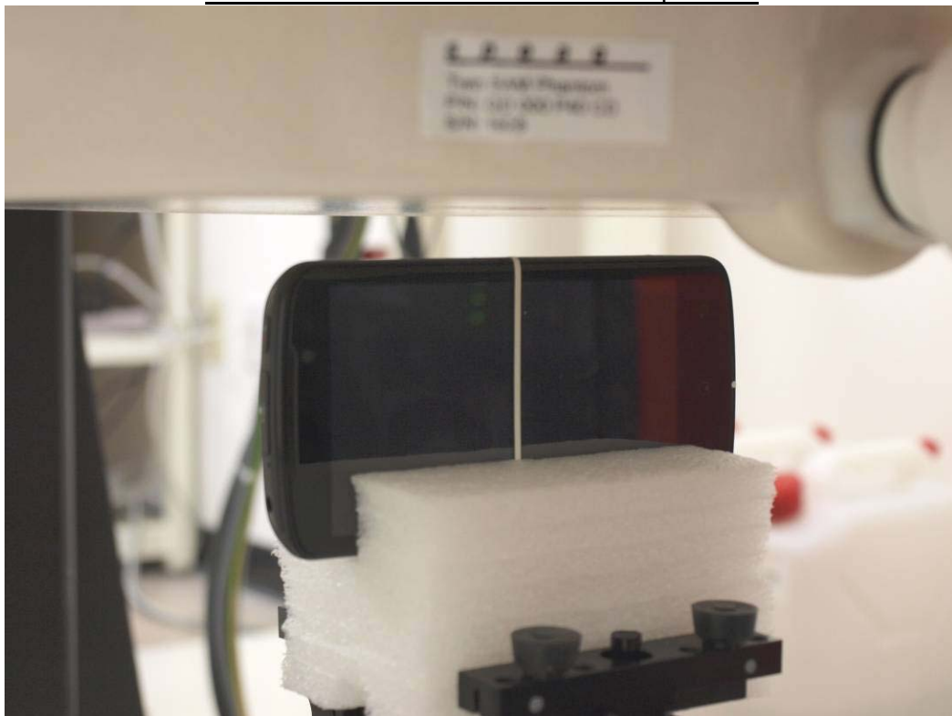
BODY – RIGHT EDGE with 10 mm Separation
