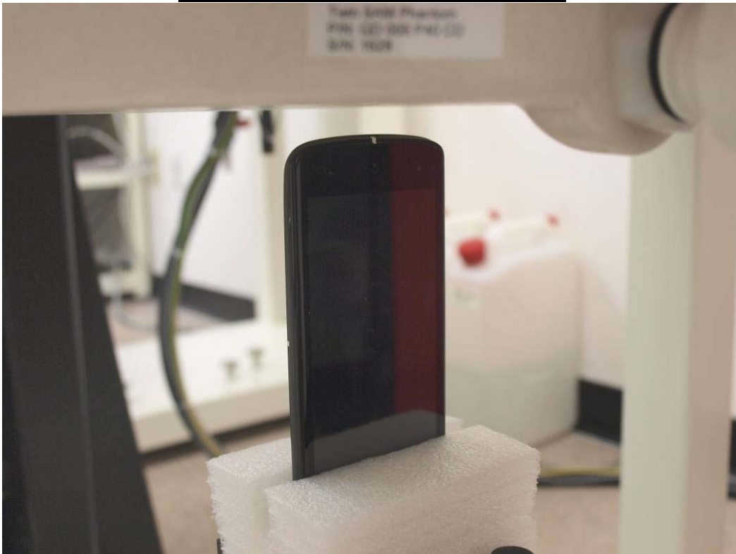
BODY – BOTTOM with 10 mm Separation
