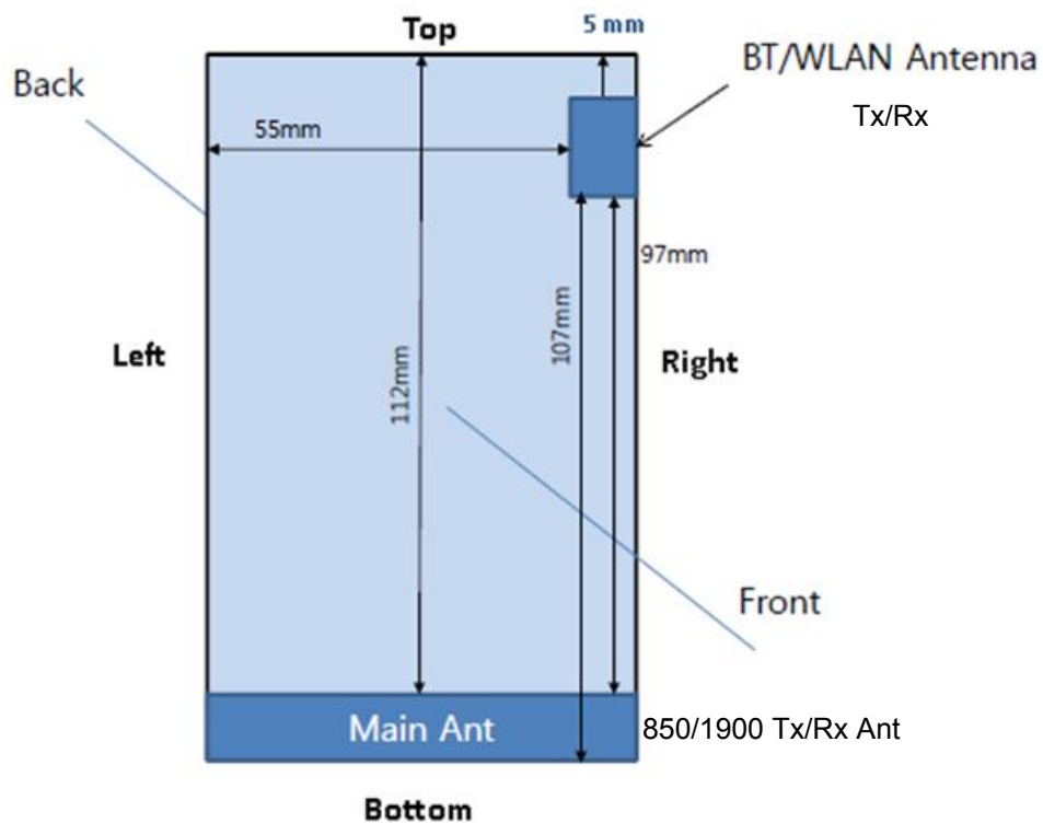
Figure 13-1 Identification of Sides for SAR Testing
