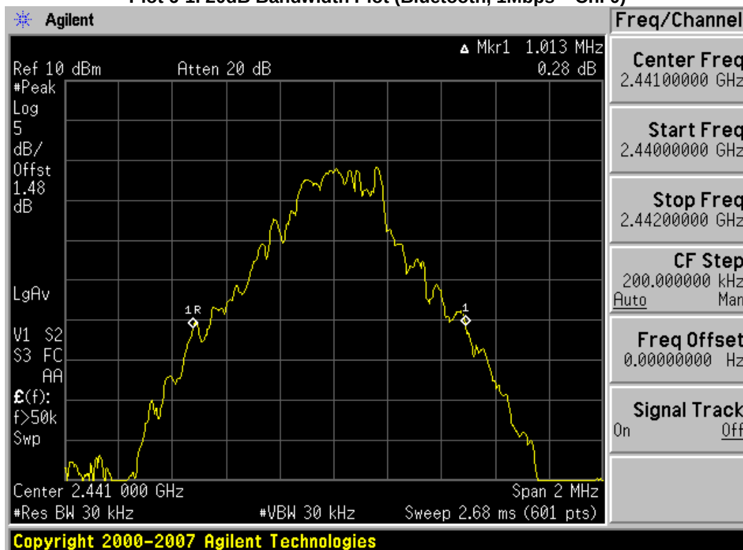
Plot 6-2. 20dB Bandwidth Plot (Bluetooth, 1Mbps – Ch. 39)
