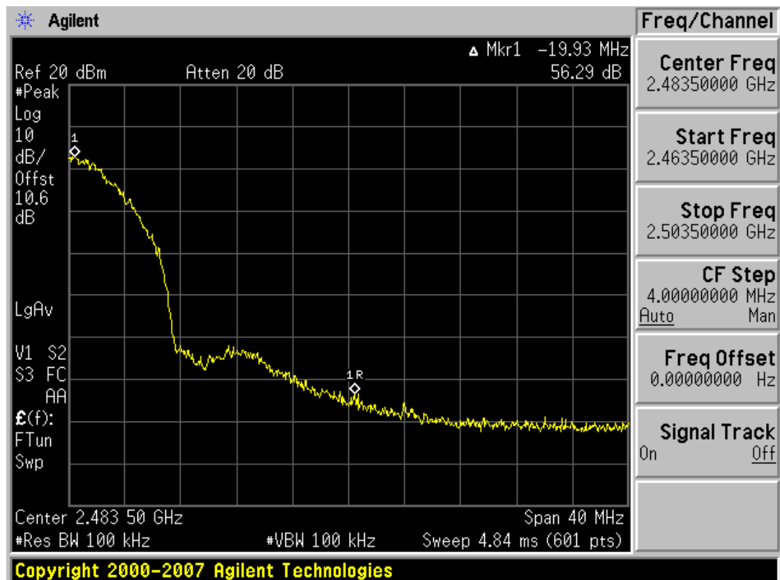
BandEdge (802.11b-CH11)
