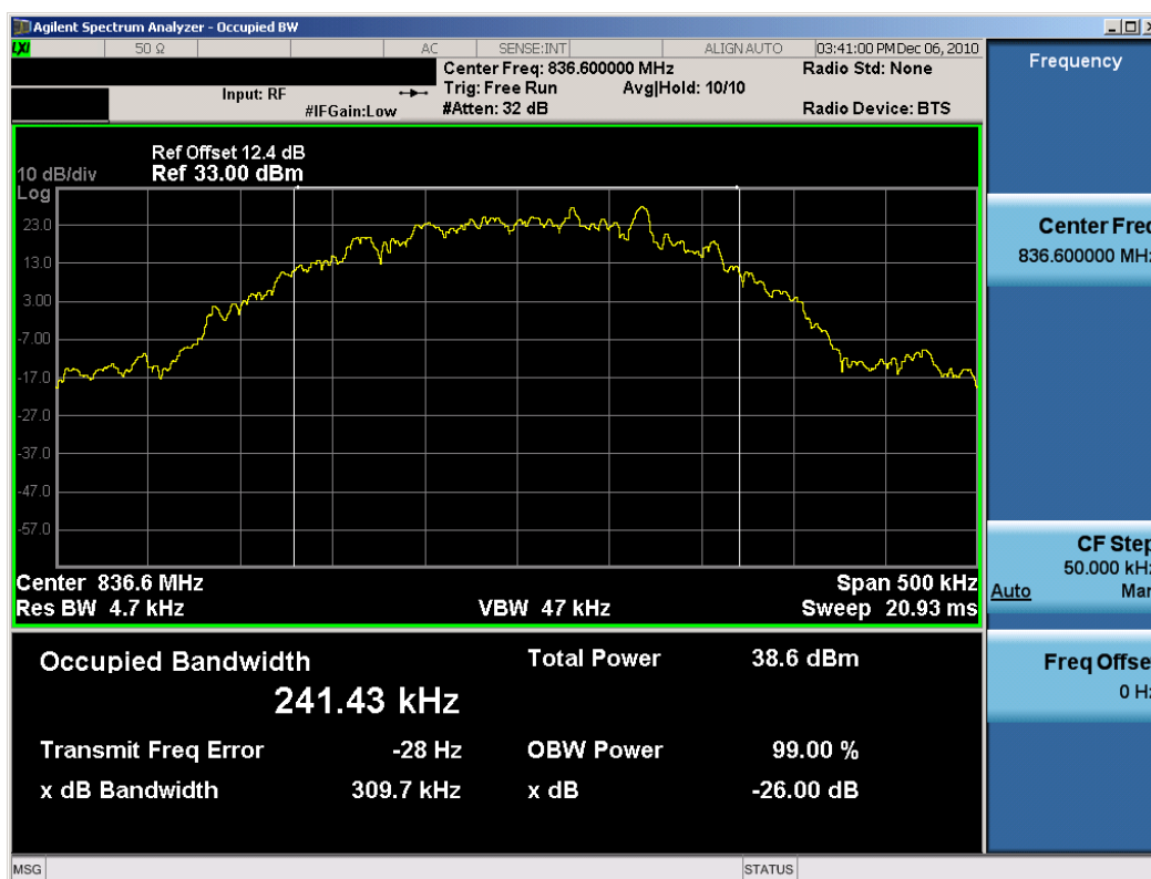
Plot 7-6. Occupied Bandwidth Plot (Cellular GSM Mode – Ch. 190)
