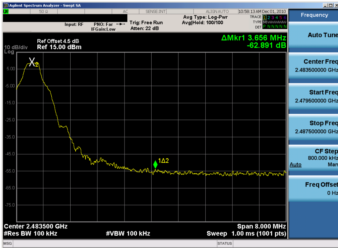
Plot 6-11. Band Edge Plot (Bluetooth, 1Mbps - Ch. 78)
