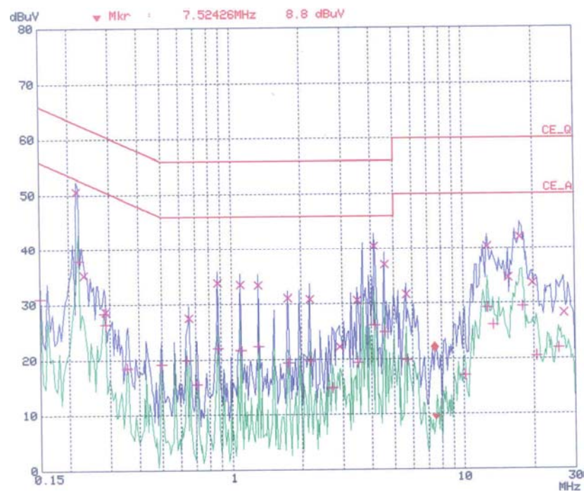
< Hot line >
