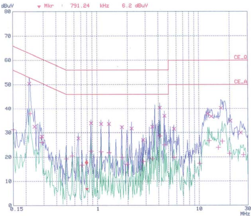
< Hot line >
