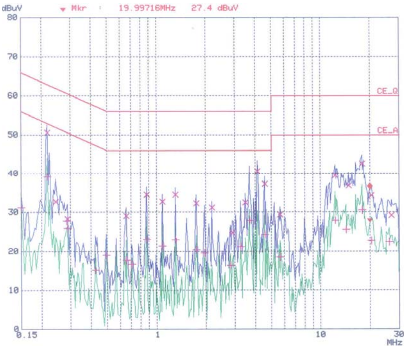
< Hot line >
