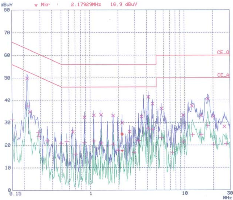
< Neutral line >
