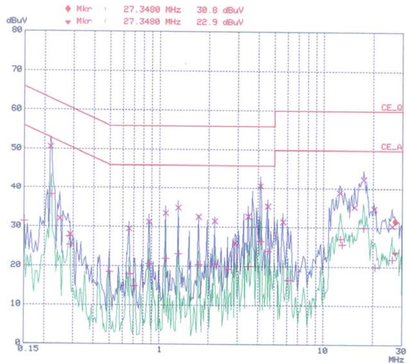
< Hot line >
