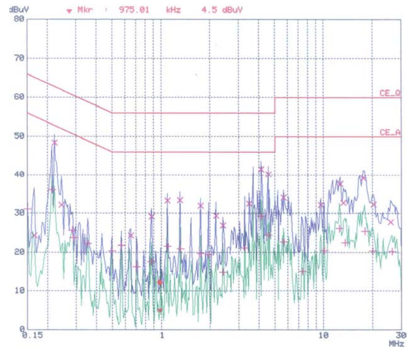
< Neutral line >
