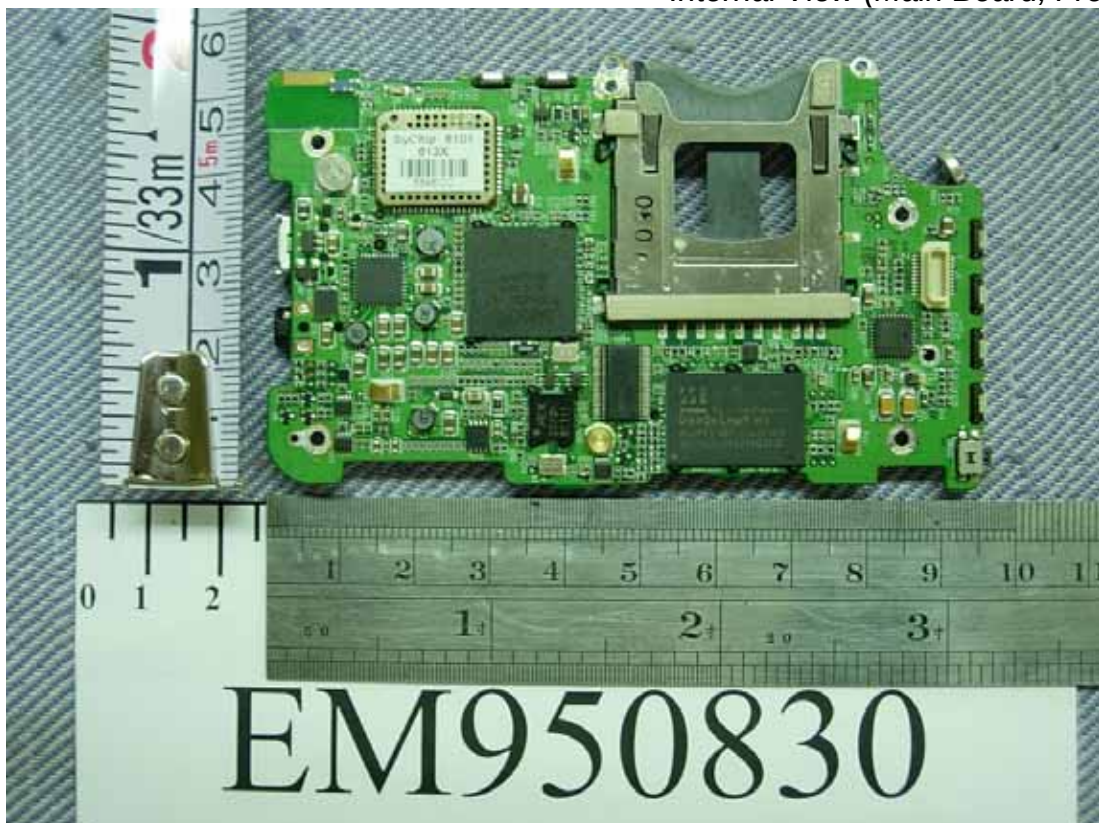
Figure 21 Internal View (Main Board, Front View)
