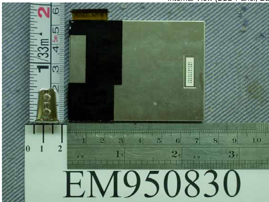
Figure 27 Internal View (LCD Panel, Back View)
