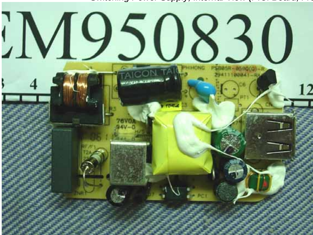
Figure 30 Switching Power Supply, Internal View (P.C. Board, Front View)
