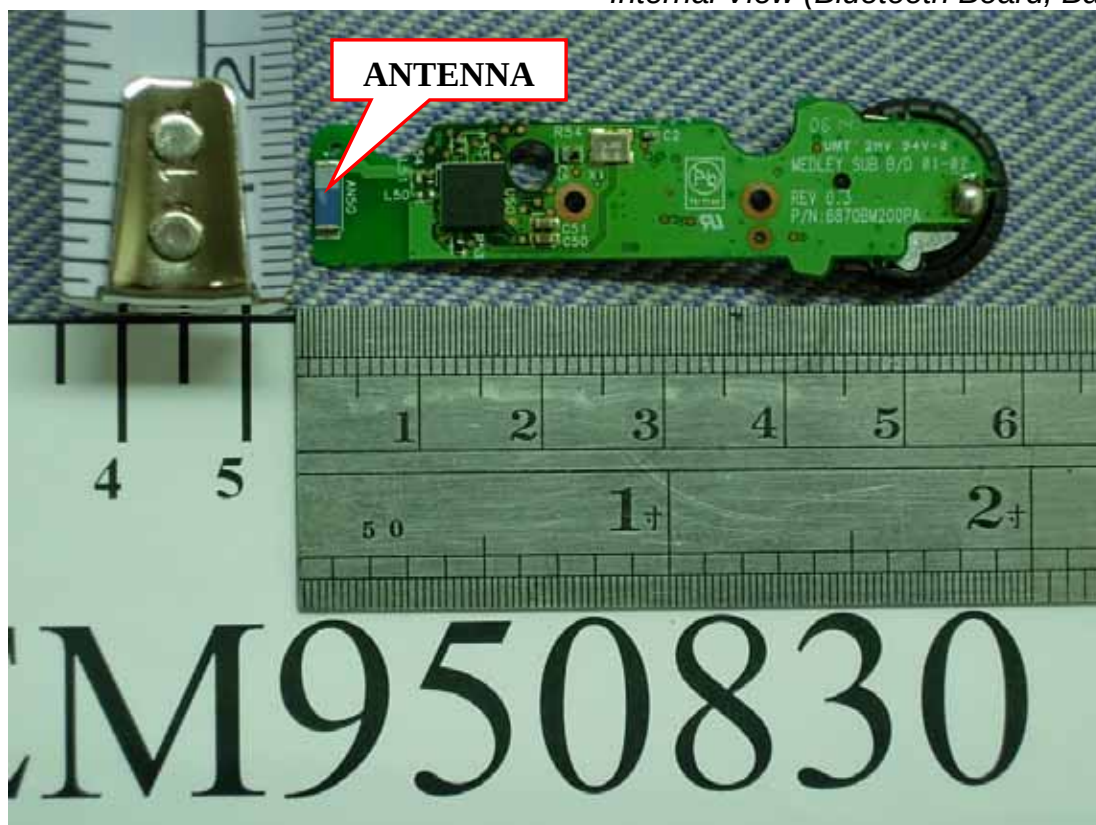
Figure 25 Internal View (Bluetooth Board, Back View)
