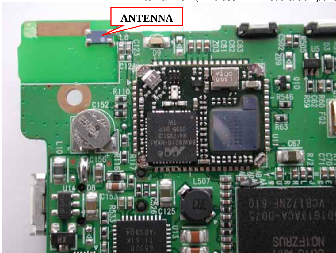
Figure 23 Internal View (Wireless LAN Module/Component View)
