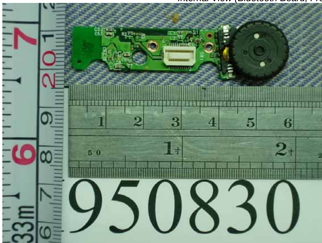
Figure 26 Internal View (Bluetooth Board, Front View)
