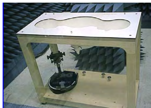
Figure 6. SAM Twin Phantom
