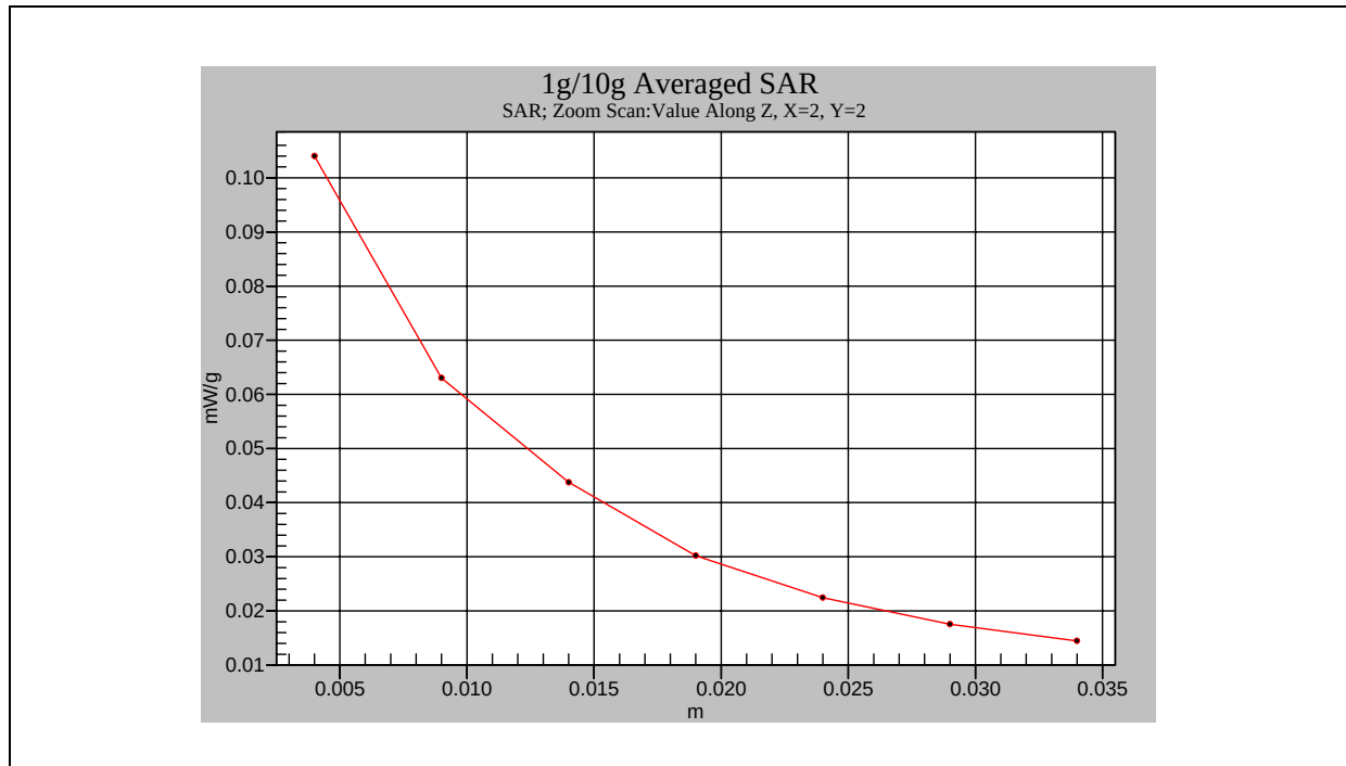
802.11b Wi-Fi Body- Channel 1_B/T on
