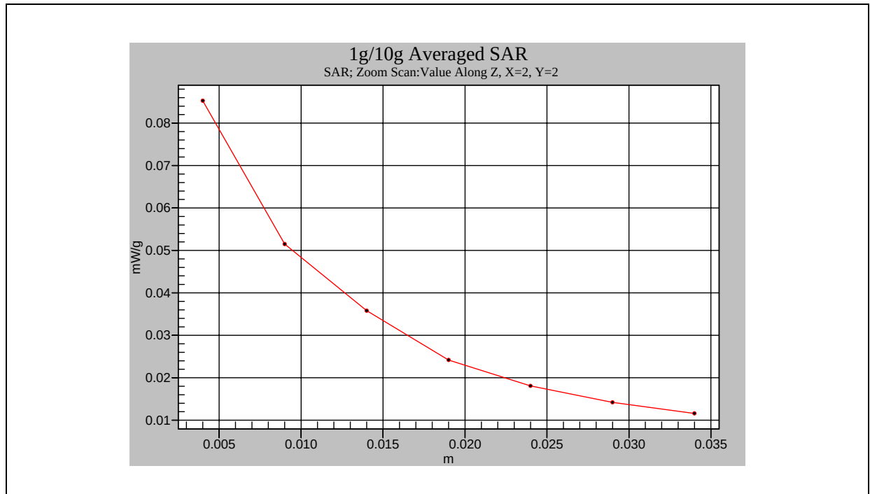
802.11b Wi-Fi Body- Channel 1 (with Top Cover) _B/T on
