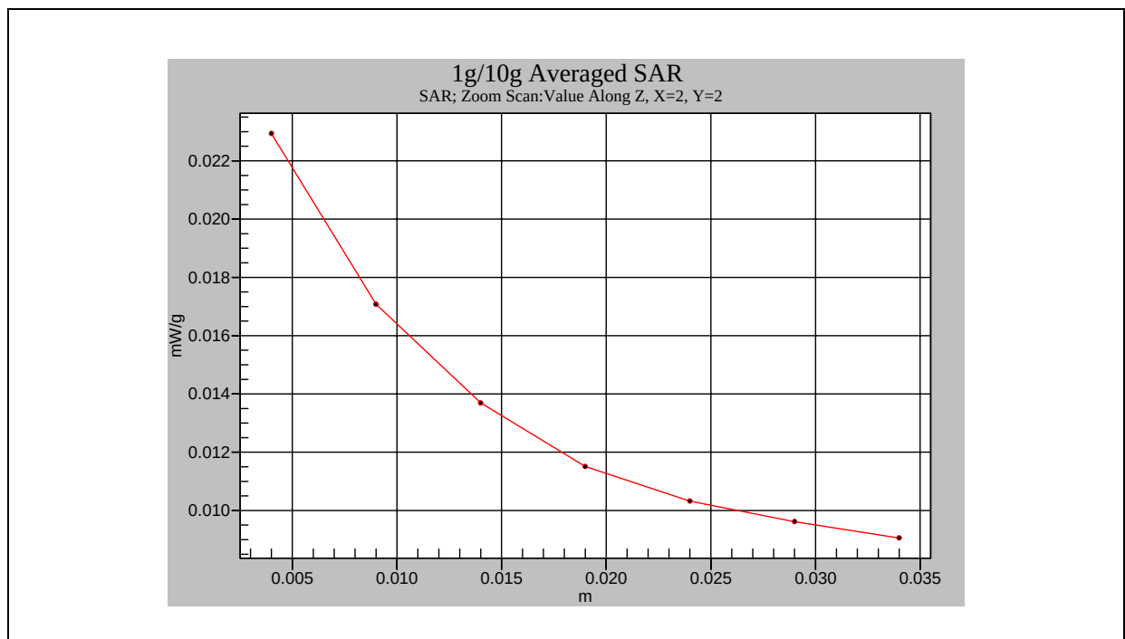
802.11g Wi-Fi Body- Channel 6 (with Top Cover)_B/T off
