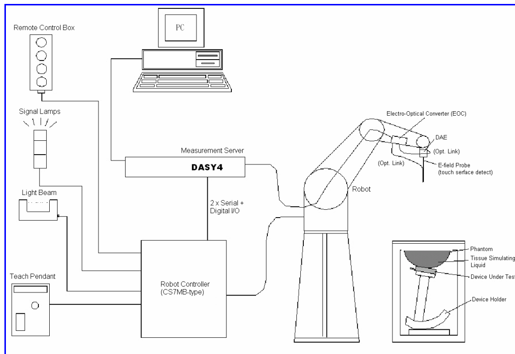
Figure 2. SAR Lab Test Measurement Setup
