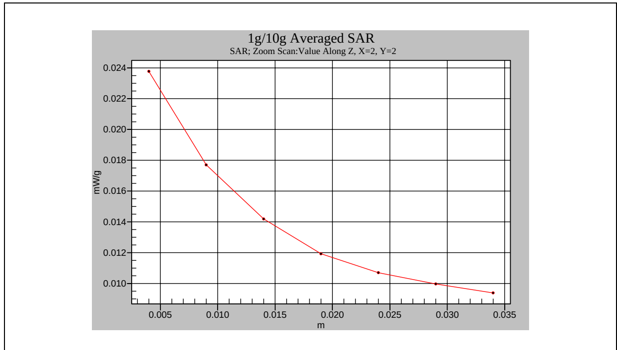
802.11g Wi-Fi Body- Channel 6 (with Top Cover)_B/T on
