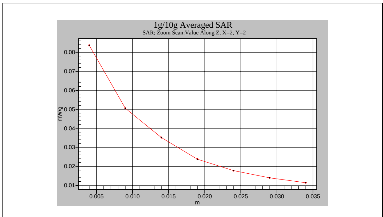
802.11b Wi-Fi Body- Channel 1 (with Top Cover) _B/T off
