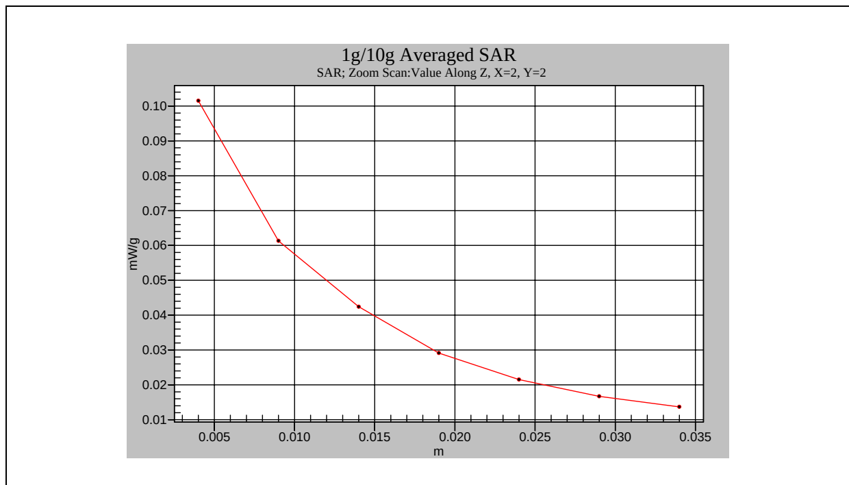
802.11b Wi-Fi Body- Channel 1_B/T off
