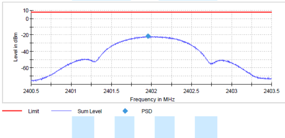
Power Density Plot on configuration : Lowest channel (2 402 MHz)
