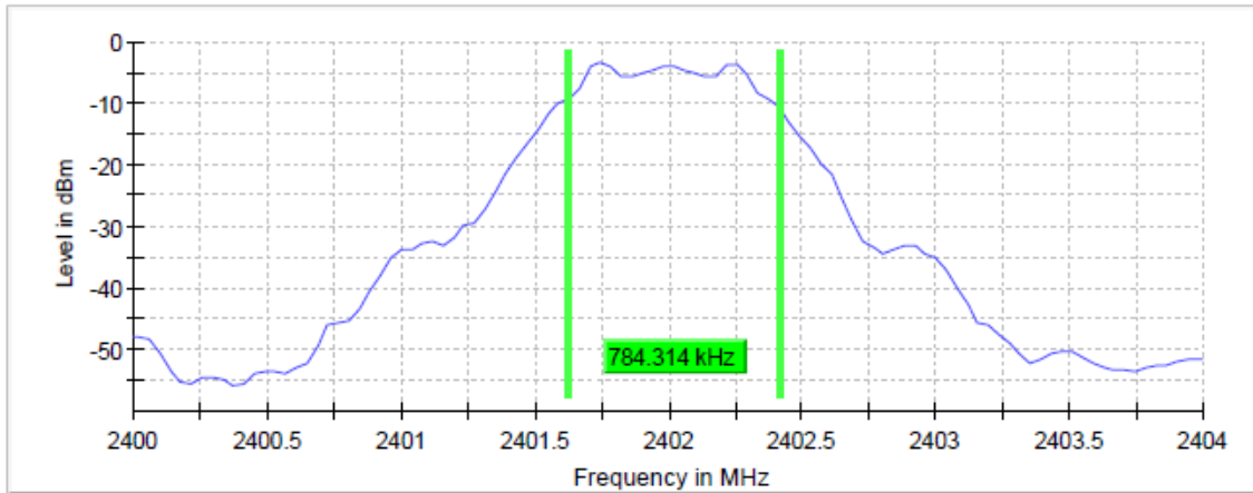
6 dB Bandwidth Plot on Configuration : Lowest channel (2 402 MHz)
