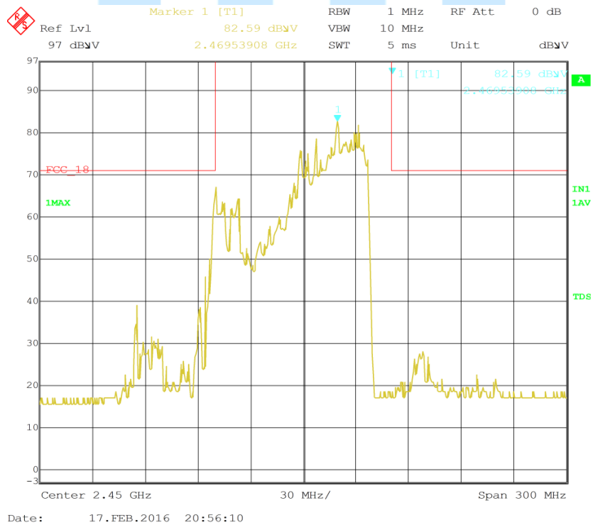
< Fig 8. Frequency Measurements (Minimum Frequency Observed: 2.469 GHz) >
