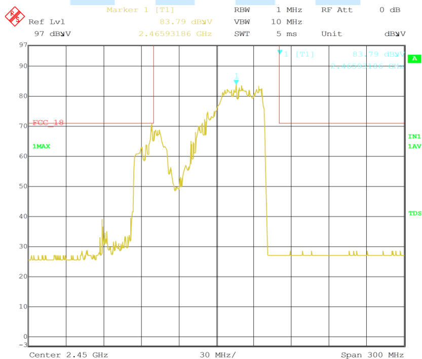
< Fig 10. Frequency Measurements (Minimum Frequency Observed: 2.465 GHz) >
