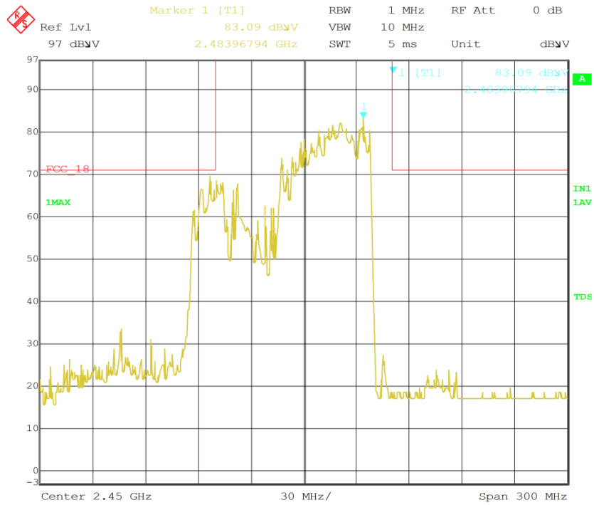
< Fig 7. Frequency Measurements (Maximum Frequency Observed: 2.483 GHz) >
