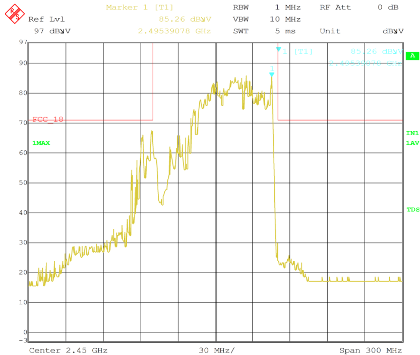
< Fig 9. Frequency Measurements (Maximum Frequency Observed: 2.495 GHz) >
