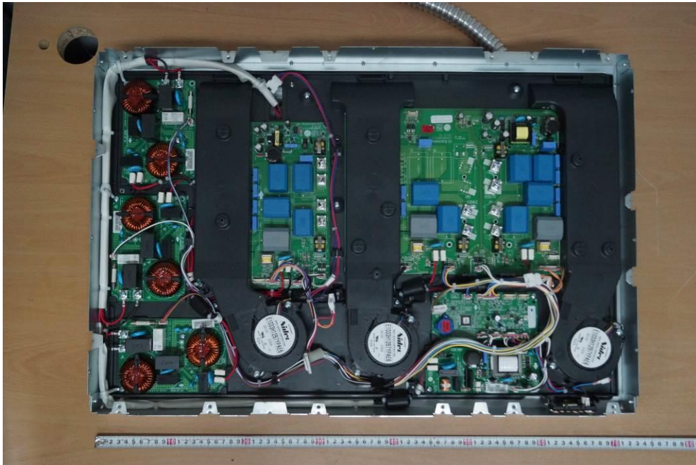
<OLD Inner of EUT >
