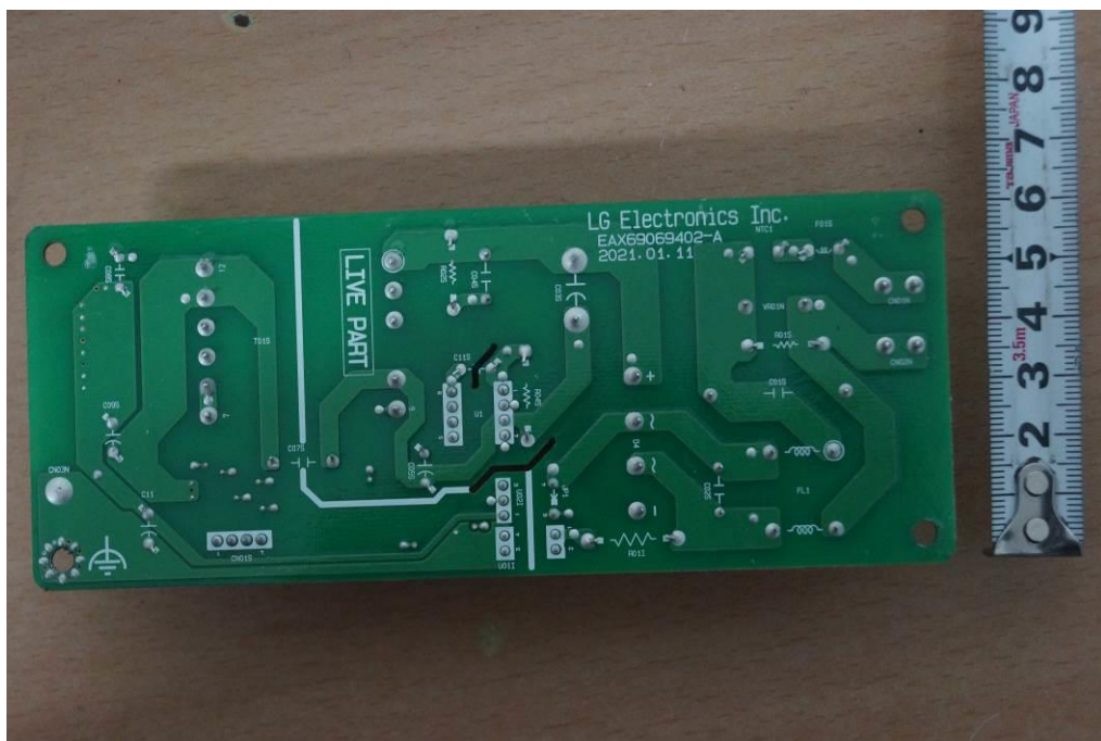
< OLD Power PCB >
