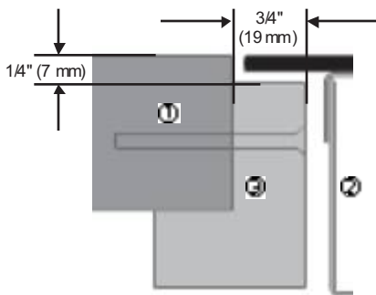
L-shaped cleat (Front and Back)
