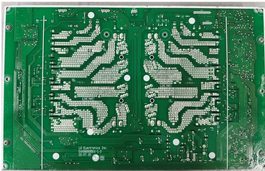
< Inverter 4B PCB (rear) >
