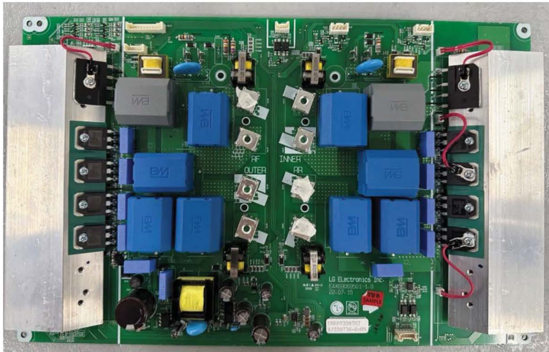
< Inverter 4B PCB (front) >
