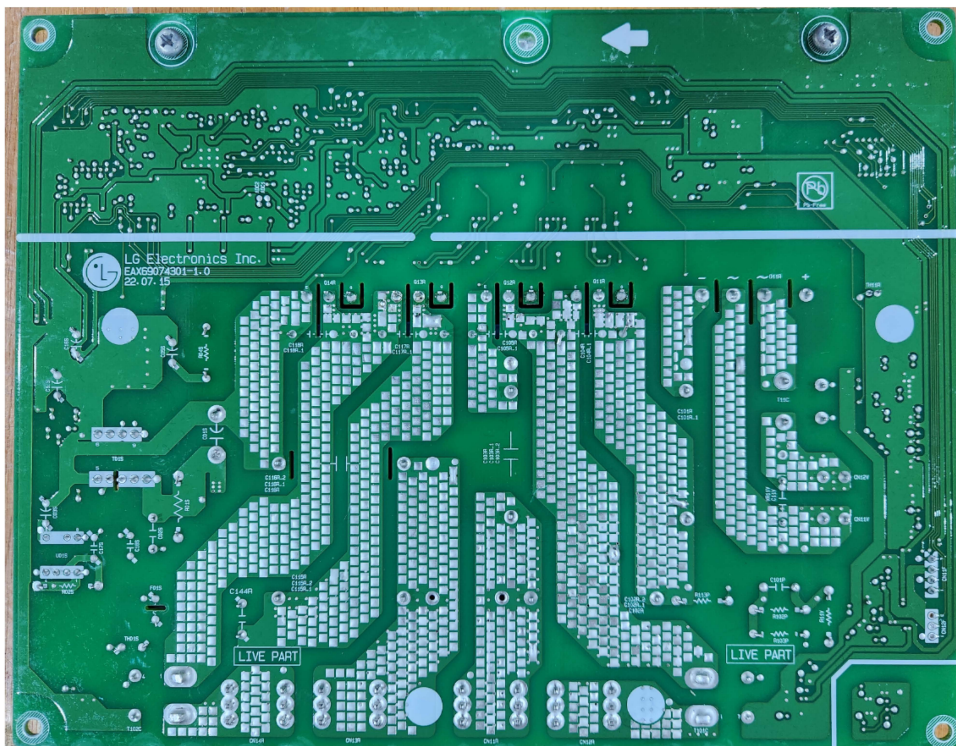
< Inverter 2B PCB (rear) >
