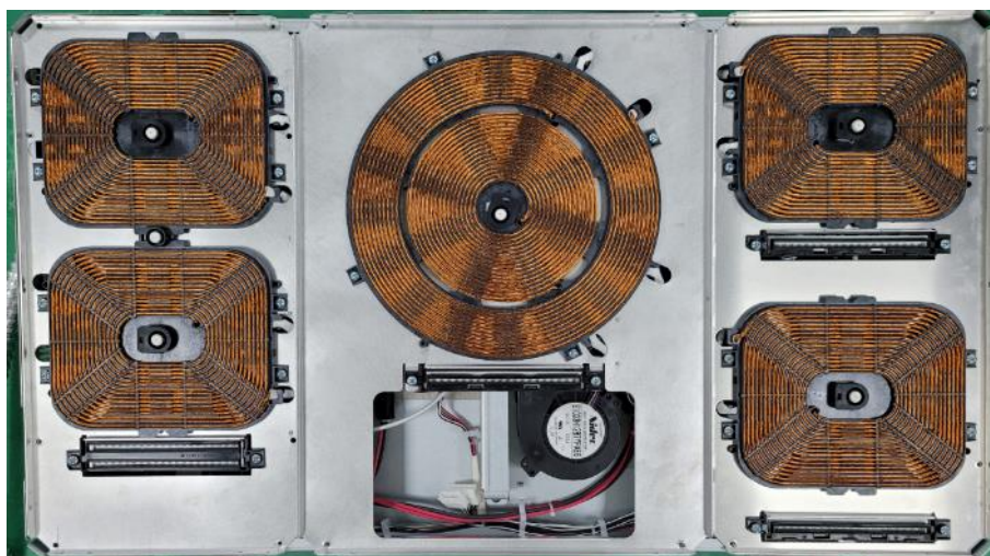
< IH core plate >
