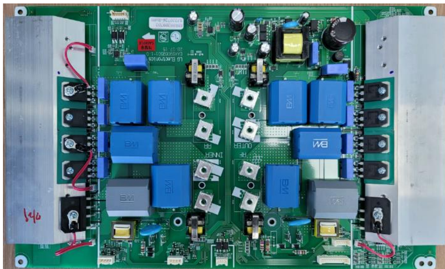
< Inverter 4B PCB (front) >
