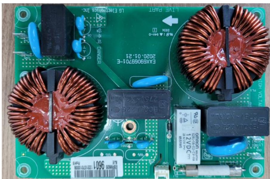
< Noise filter PCB (front) >
