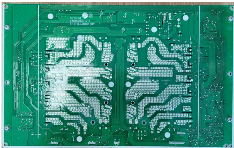
< Inverter 4B PCB (rear) >
