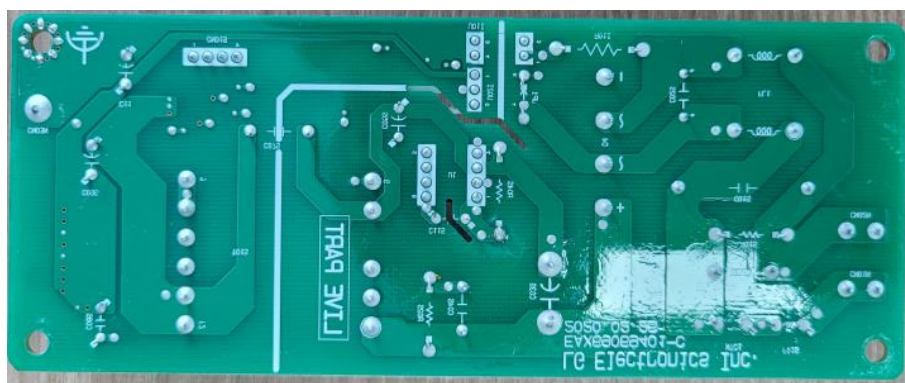
< Power(SMPS) PCB (rear) >
