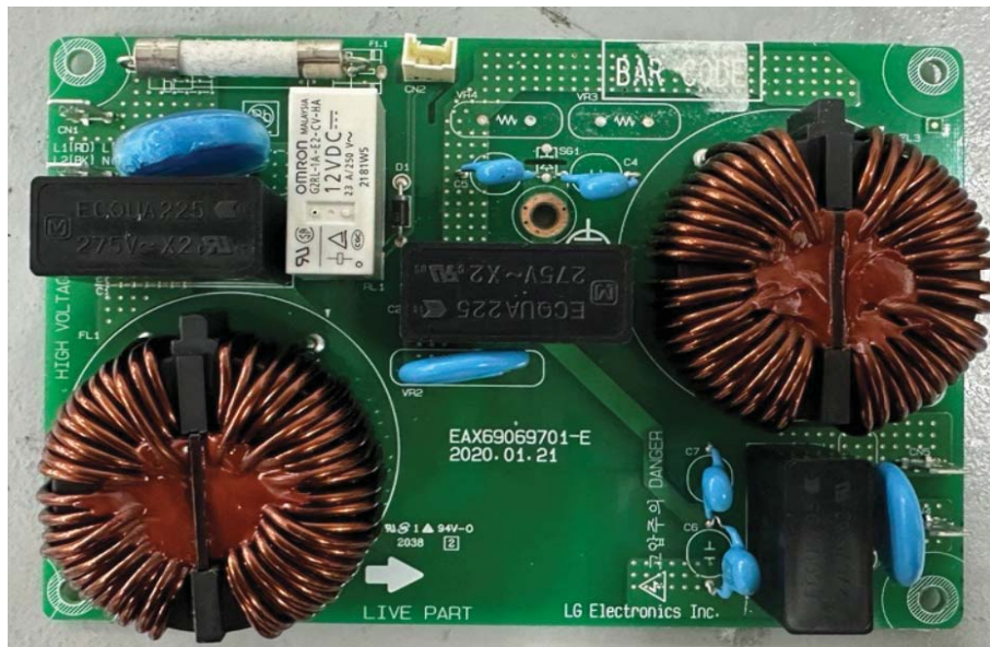
< Noise filter PCB (front) >
