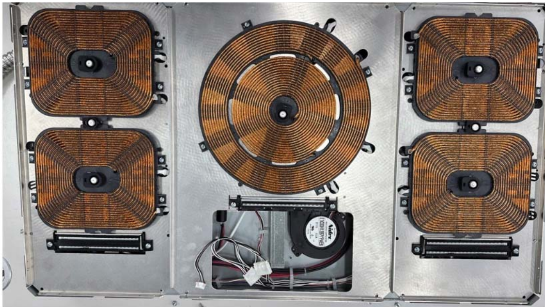
< IH core plate >
