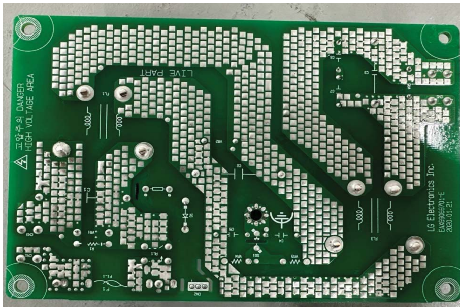
< Noise filter PCB (rear) >
