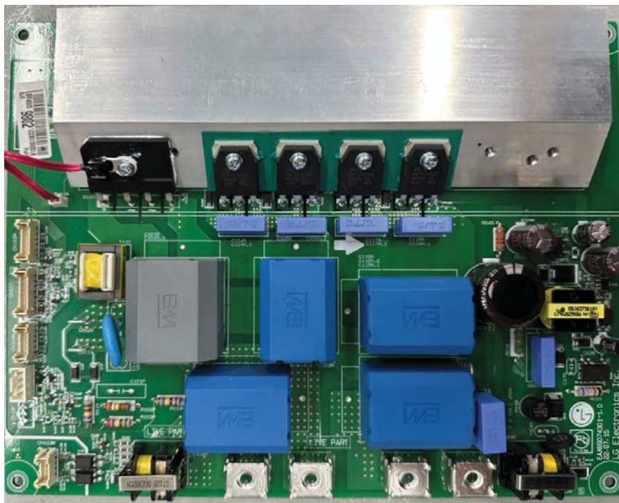
< Inverter 2B PCB (front) >
