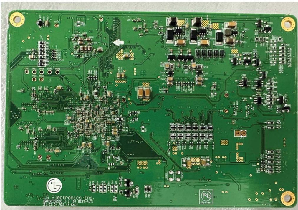
< TFT LCD PCB (rear) >
