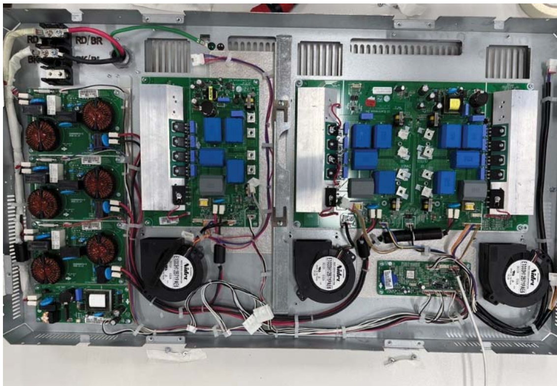
< Bottom plate >
