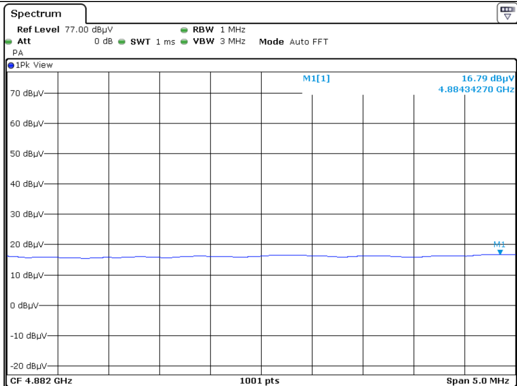
Middle Channel_H_Peak
