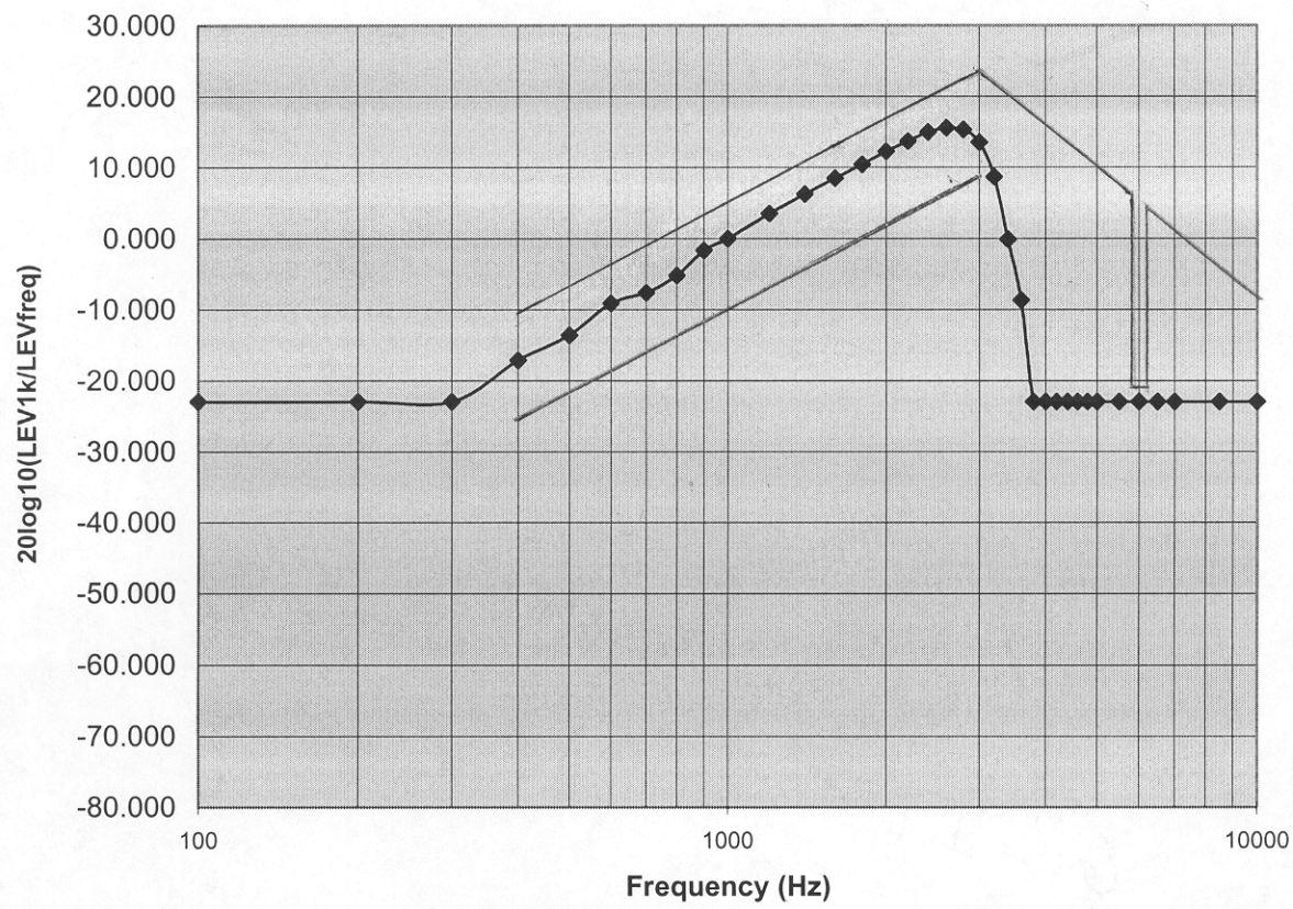
Mid Channel --- Audio Frequency Response De-Emphasis circuit off
