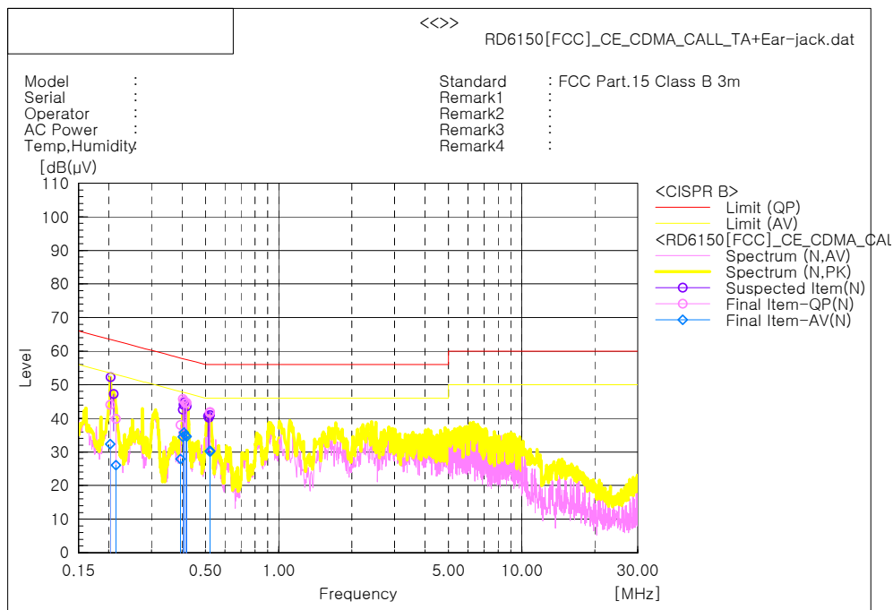
Plot 7-1. Line-Conducted Test Plot.
