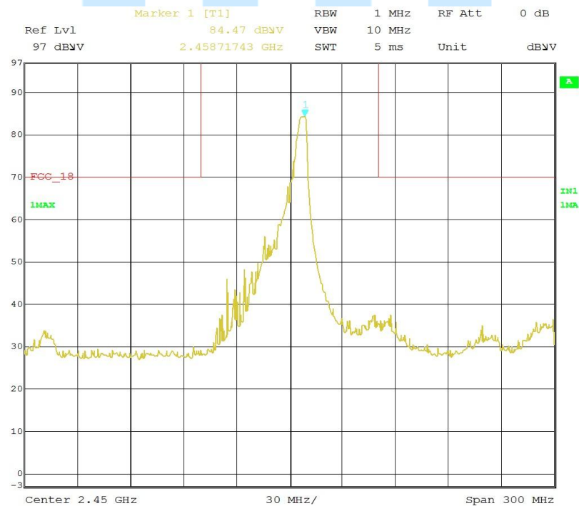
< Fig 10. Frequency Measurements (Minimum Frequency Observed: 2.458 GHz) >
