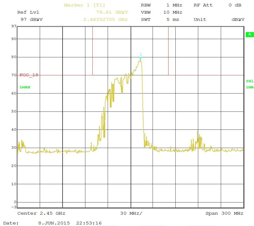
< Fig 7. Frequency Measurements (Maximum Frequency Observed: 2.463 GHz) >
