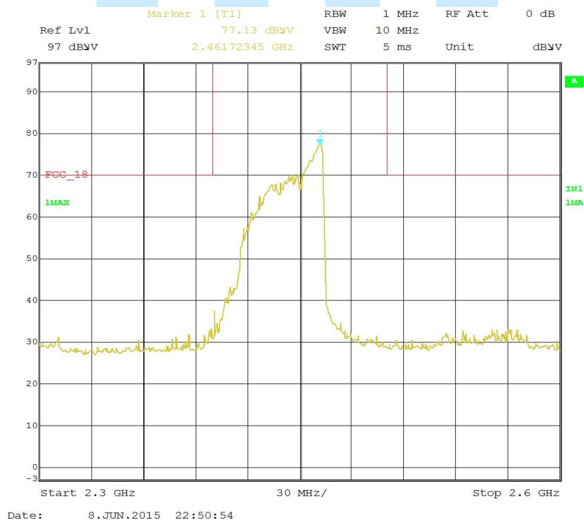
< Fig 8. Frequency Measurements (Minimum Frequency Observed: 2.461 GHz) >
