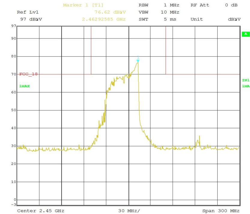
< Fig 9. Frequency Measurements (Maximum Frequency Observed: 2.462 GHz) >
