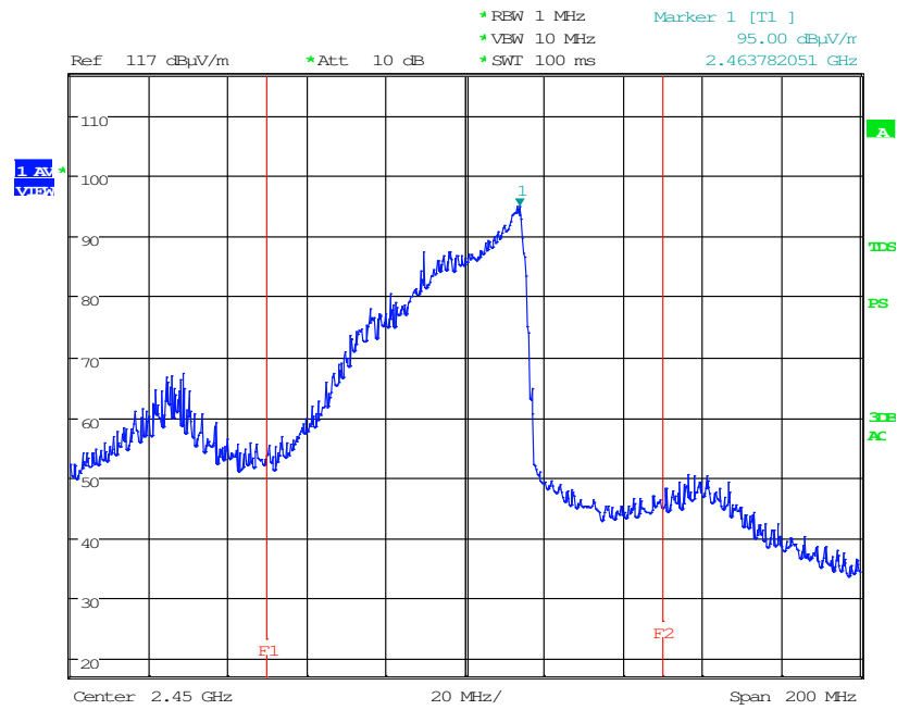
< Fig 7. Frequency Measurements (Maximum Frequency Observed: 2.463 GHz) >
