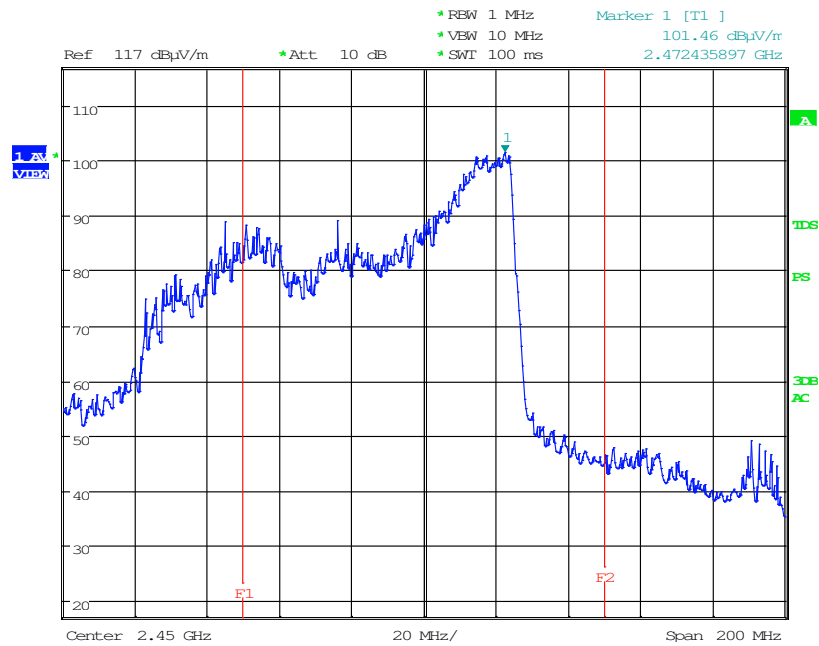
< Fig 9. Frequency Measurements (Maximum Frequency Observed: 2.472 GHz) >
