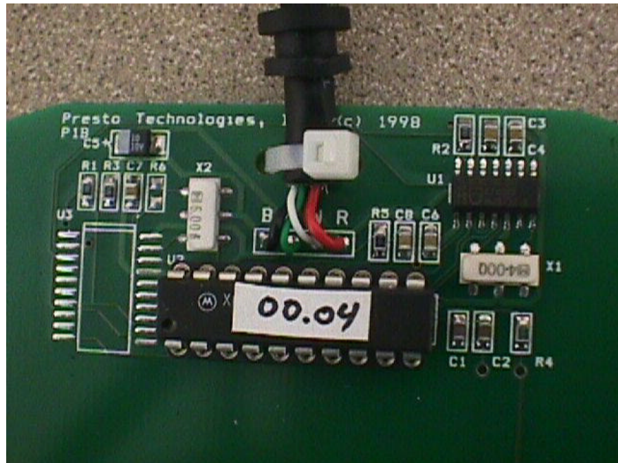
FIGURE 3: Mousepad Micro Processor Hitag Reader Chip Component Side
