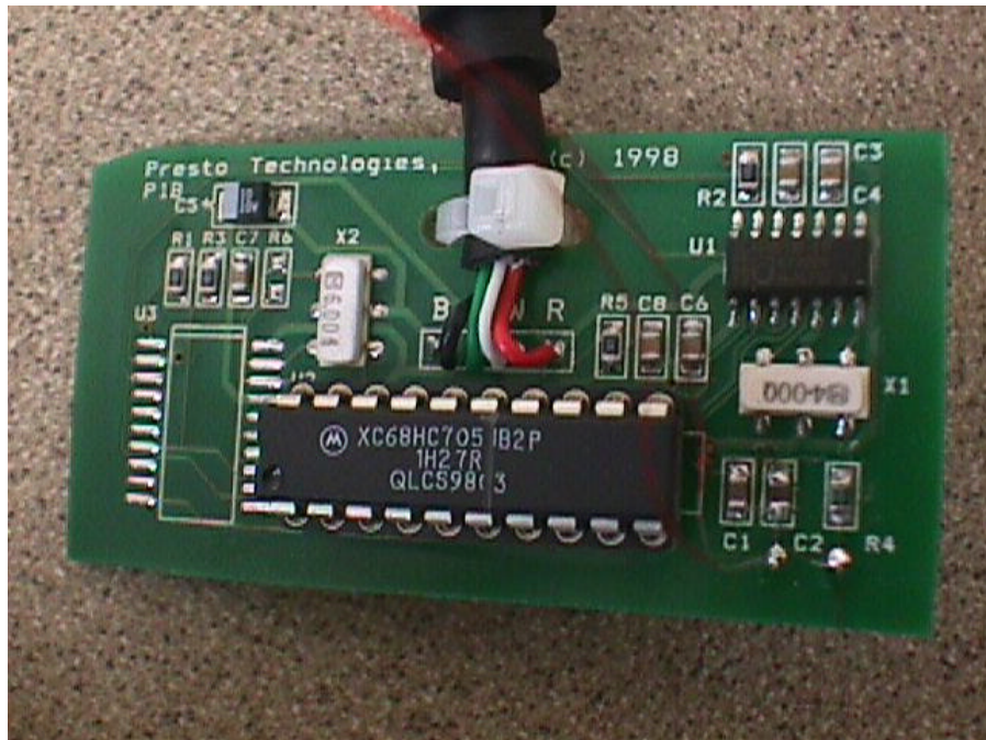
FIGURE 17: Mousepad prototype Micro Processor Hitag Reader Chip Component Side
