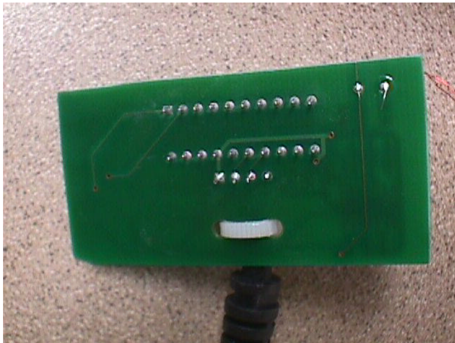
FIGURE 18: Mousepad prototype Solder Side Micro Processor Hitag Reader Chip PCB
