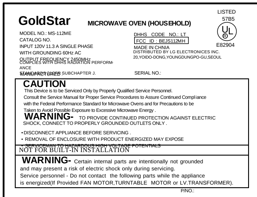
<Fig. 1. Sample Label of Nameplate>
