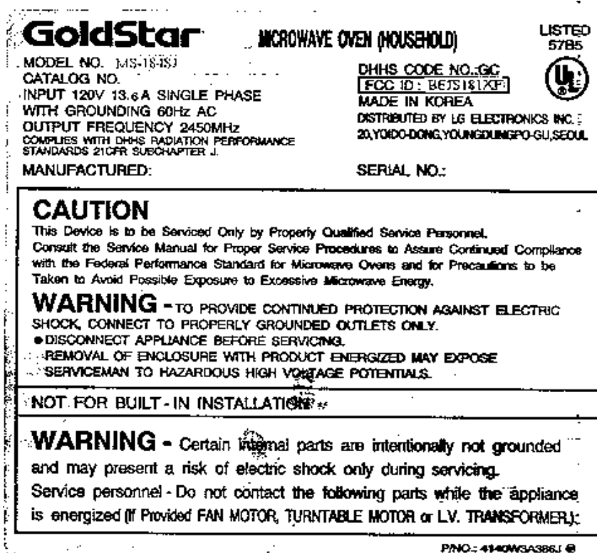
LABEL LOCATION (2) – ALTERNATE LOCATION
