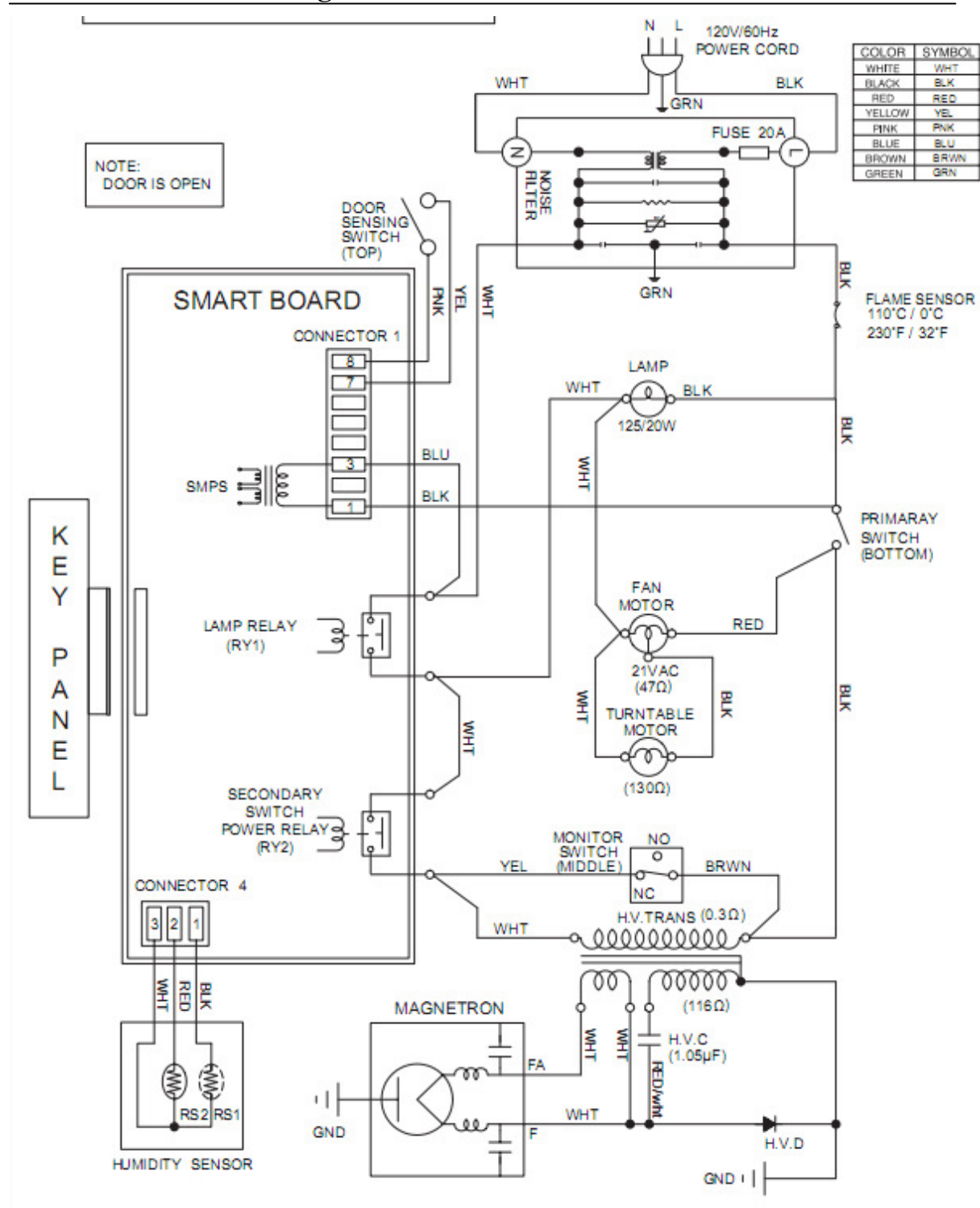
<Fig. 1-1. Block Diagram>
