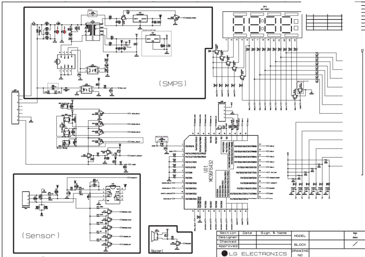
<Fig. 1-2. Schematic Diagram – Main board>
