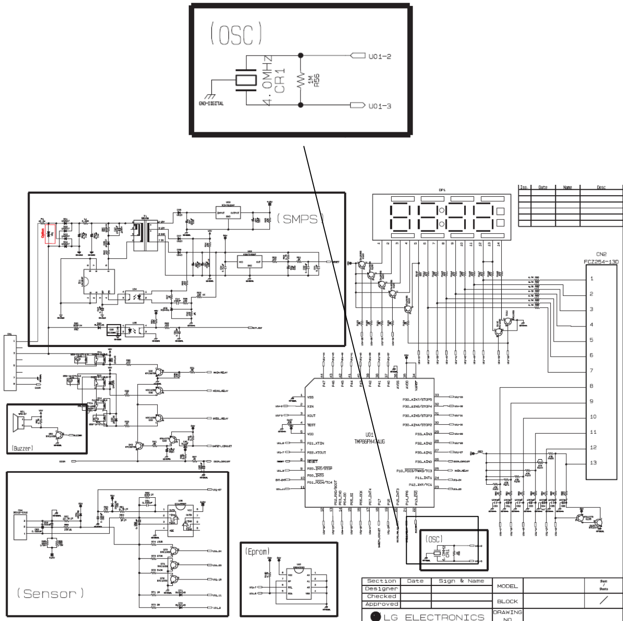
<Fig. 4. PCB Circuit Diagram>
