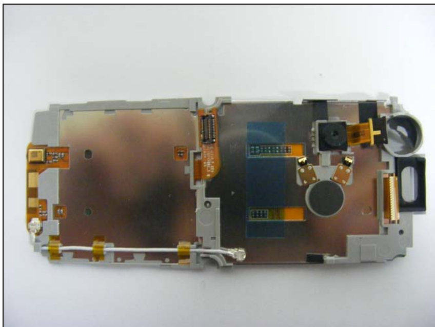
Bottom view of LCD Panel and Key Pad
