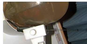
Fig. 14 Head SAR Test Setup
