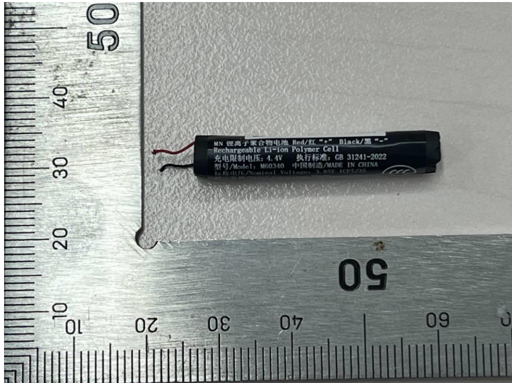
Fig. 9 Battery view
