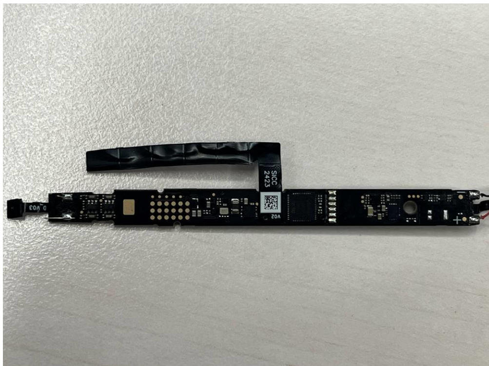
Fig. 8 PCB view 2
