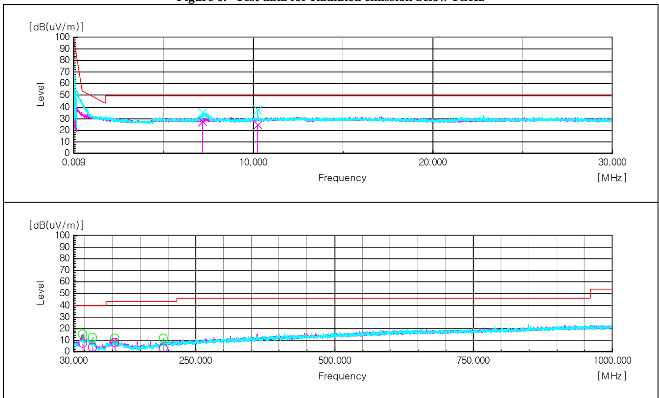
Figure 6. Test data for Radiated emission below 1GHz
