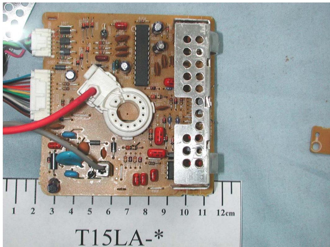
FIGURE 8 COLOR MONITOR (M/N: T15LA-*) TUBE BOARD (COMPONENT SIDE)
