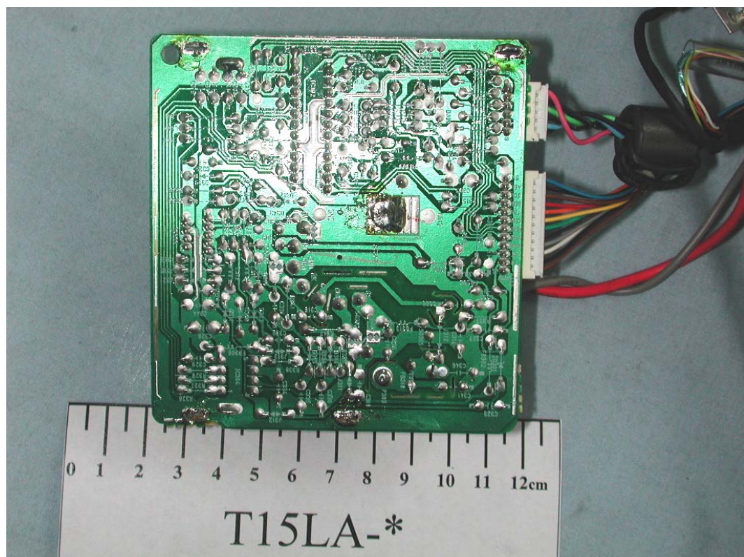
FIGURE 9 COLOR MONITOR (M/N: T15LA-*) TUBE BOARD (SOLDERED SIDE)
