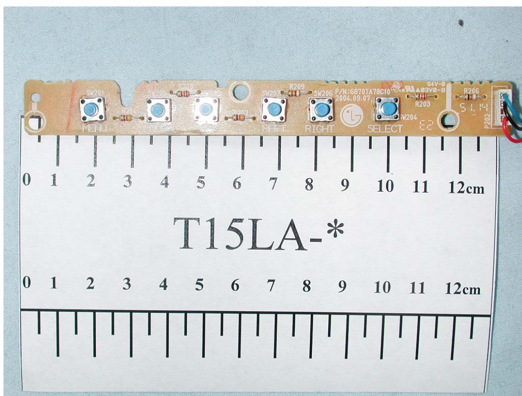
FIGURE 6 COLOR MONITOR (M/N: T15LA-*) OPERATION BOARD (COMPONENT SIDE)
