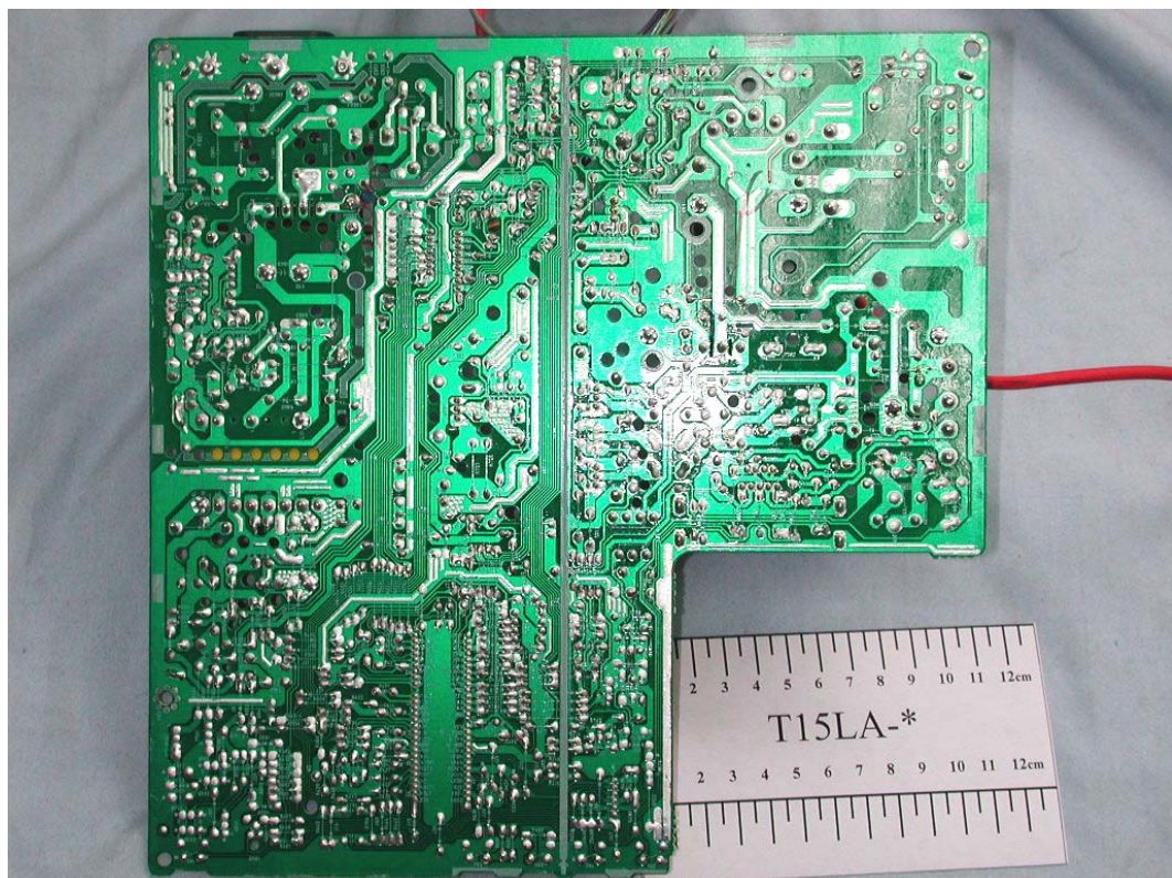
FIGURE 3 COLOR MONITOR (M/N: T15LA-*) MAIN BOARD (SOLDERED SIDE)
