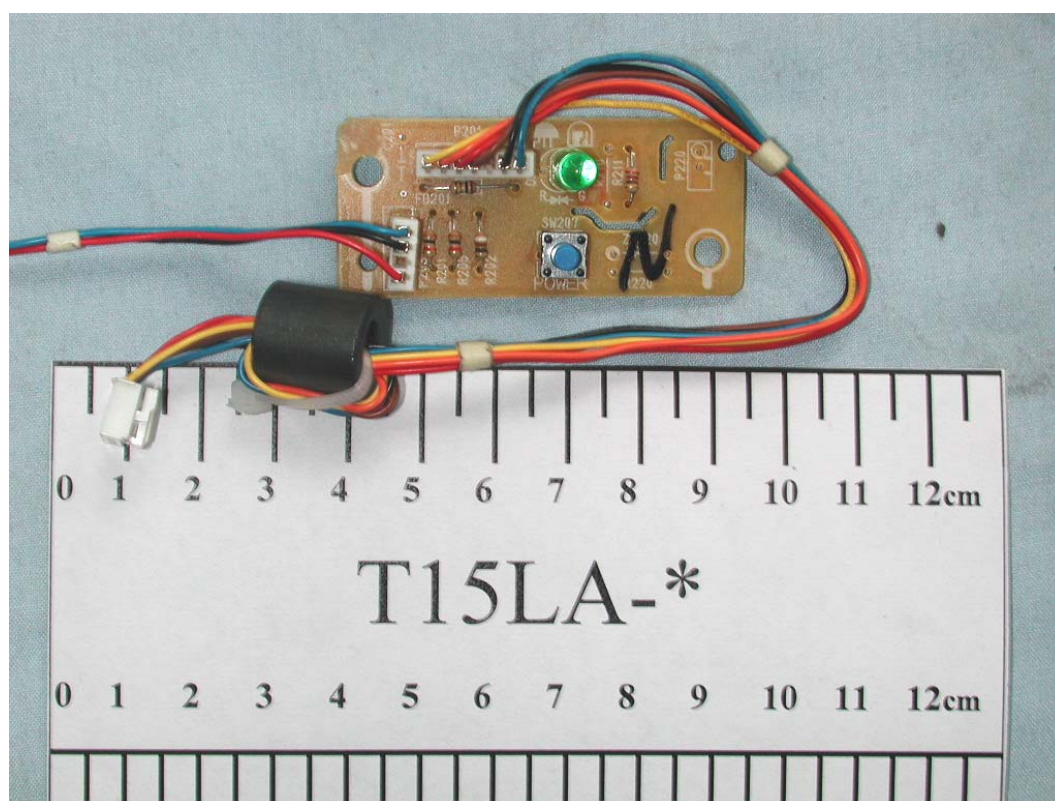
FIGURE 4 COLOR MONITOR (M/N: T15LA-*) POWER BUTTON BOARD (COMPONENT SIDE)
