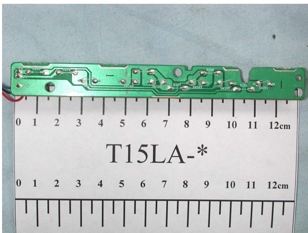
FIGURE 7 COLOR MONITOR (M/N: T15LA-*) OPERATION BOARD (SOLDERED SIDE)
