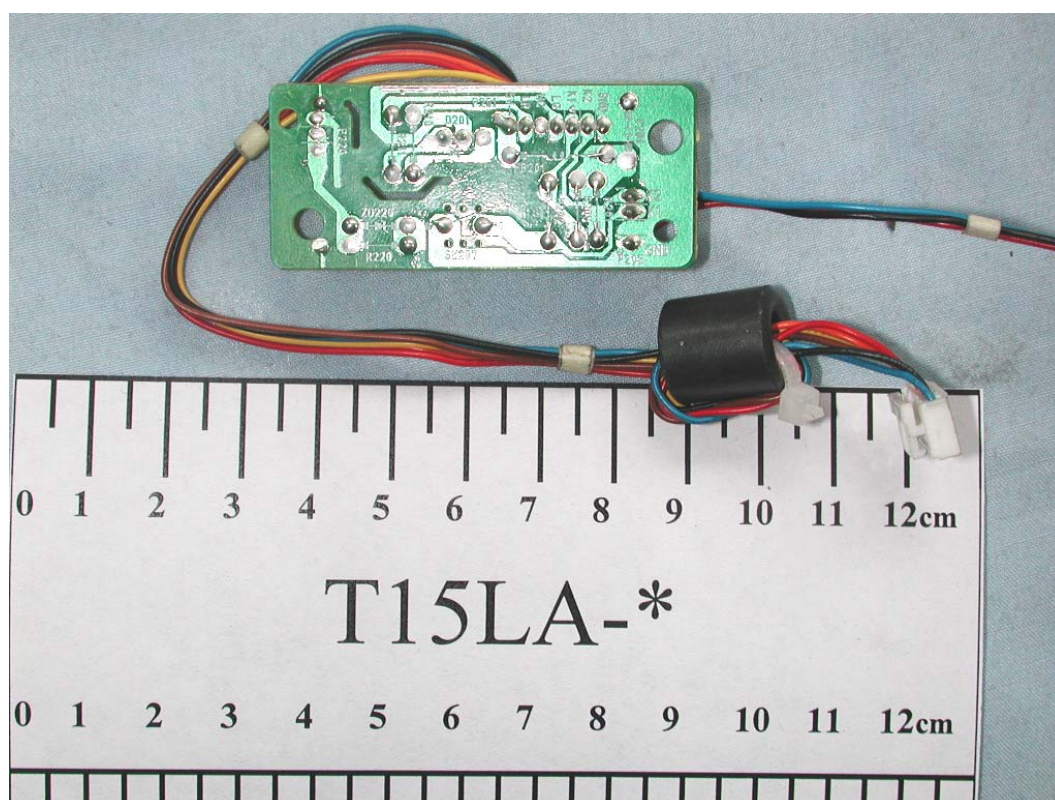
FIGURE 5 COLOR MONITOR (M/N: T15LA-*) POWER BUTTON BOARD (SOLDERED SIDE)
