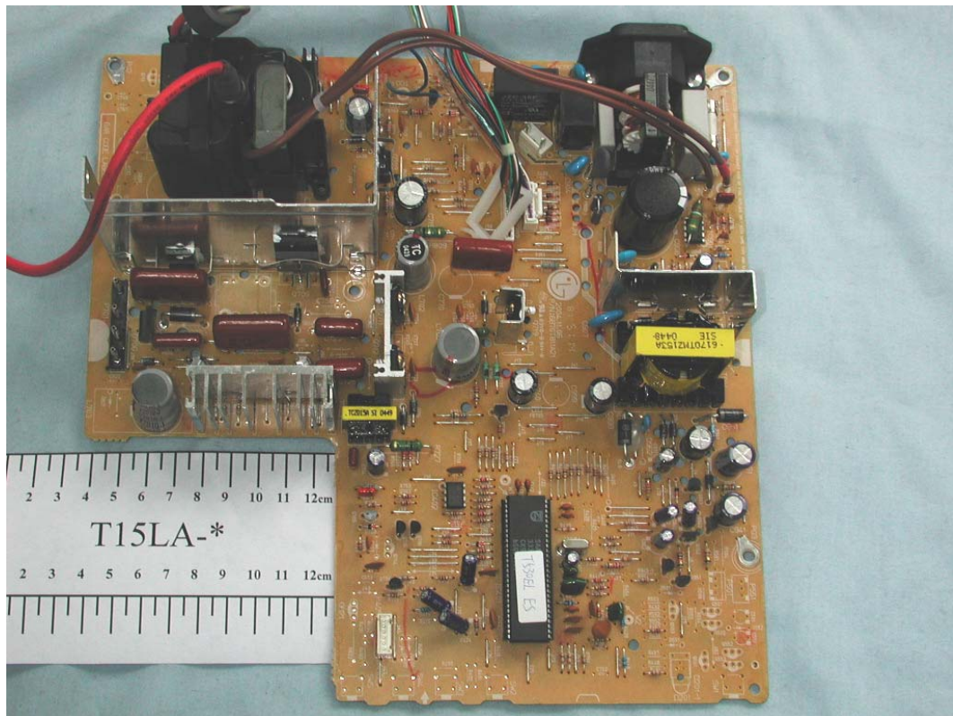
FIGURE 2 COLOR MONITOR (M/N: T15LA-*) MAIN BOARD (COMPONENT SIDE)
