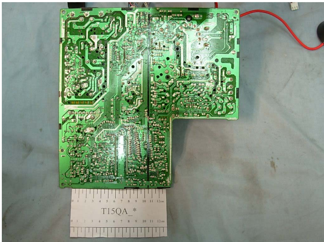
FIGURE 9 CRT MONITOR (M/N: T15QA-*) MAIN BOARD 1 (SOLDERED SIDE)
