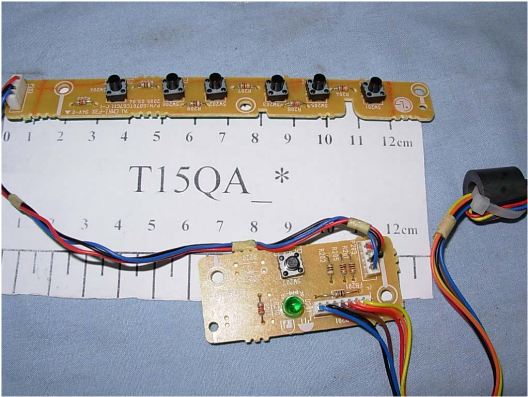
FIGURE 6 CRT MONITOR (M/N: T15QA-*) CONTROL BOARD (COMPONENT SIDE)
