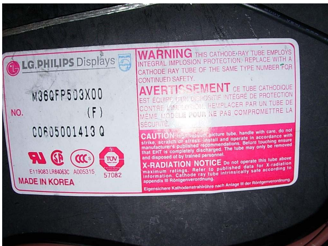
FIGURE 15 CRT MONITOR (M/N: T15QA-*) CRT LABEL
