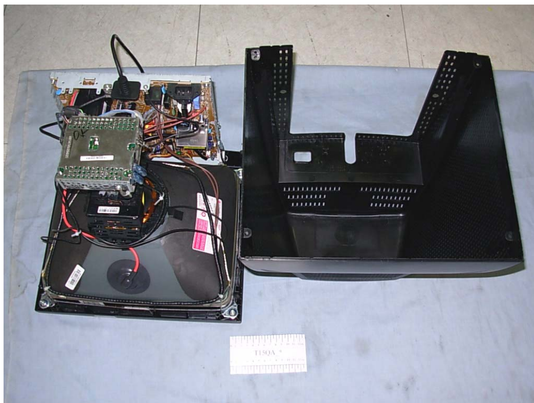
FIGURE 4 CRT MONITOR (M/N: T15QA-*) COVER REMOVED
