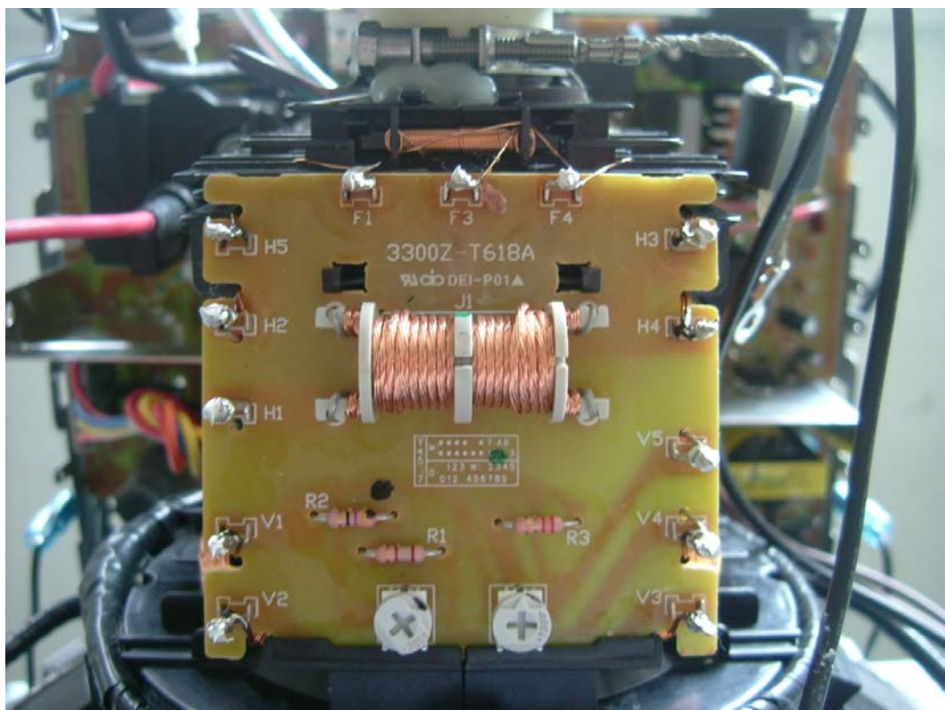
FIGURE 13 CRT MONITOR (M/N: T15QA-*) MAIN BOARD 3 COVER REMOVED
