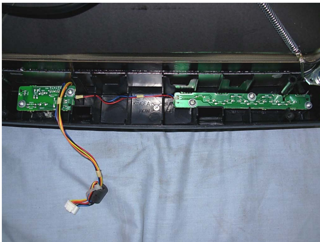
FIGURE 5 CRT MONITOR (M/N: T15QA-*) CONTROL BOARD (BACK VIEW)
