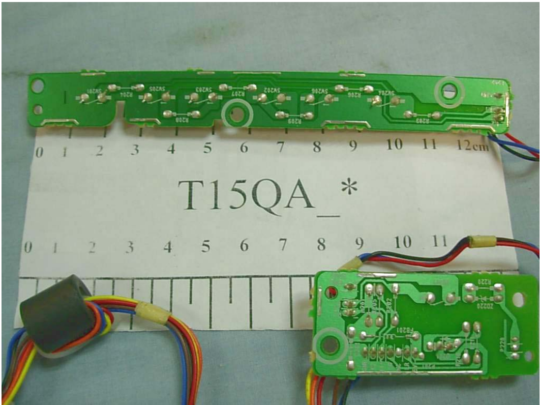
FIGURE 7 CRT MONITOR (M/N: T15QA-*) CONTROL BOARD (SOLDERED SIDE)
