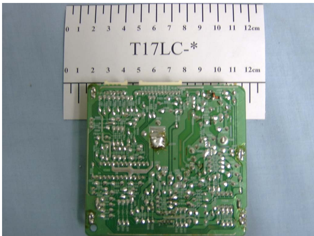
FIGURE 7 COLOR MONITOR (M/N:T17LC-*) CRT BOARD (SOLDERED SIDE)
