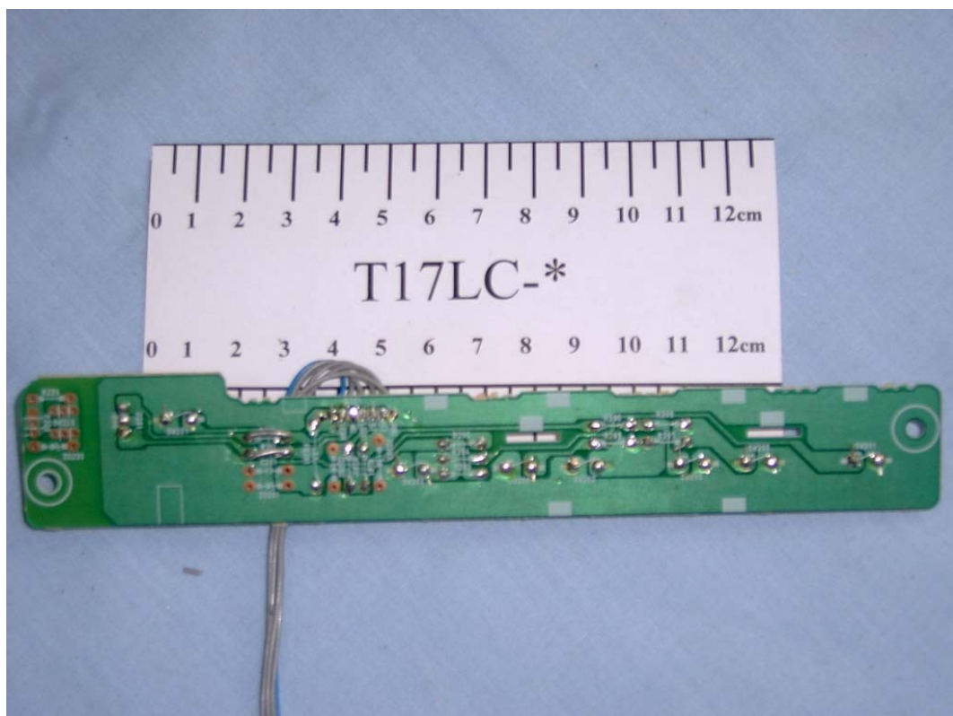
FIGURE 9 COLOR MONITOR (M/N:T17LC-*) CONTROL PANEL BOARD (SOLDERED SIDE)
