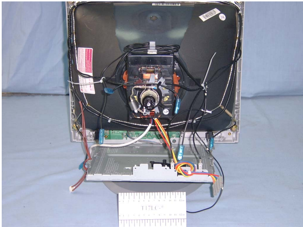
FIGURE 3 COLOR MONITOR (M/N:T17LC-*) CRT TUBE
