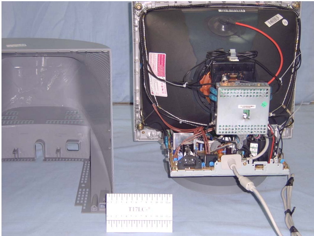
FIGURE 1 COLOR MONITOR (M/N:TI7LC-*) COVER REMOVED 1
