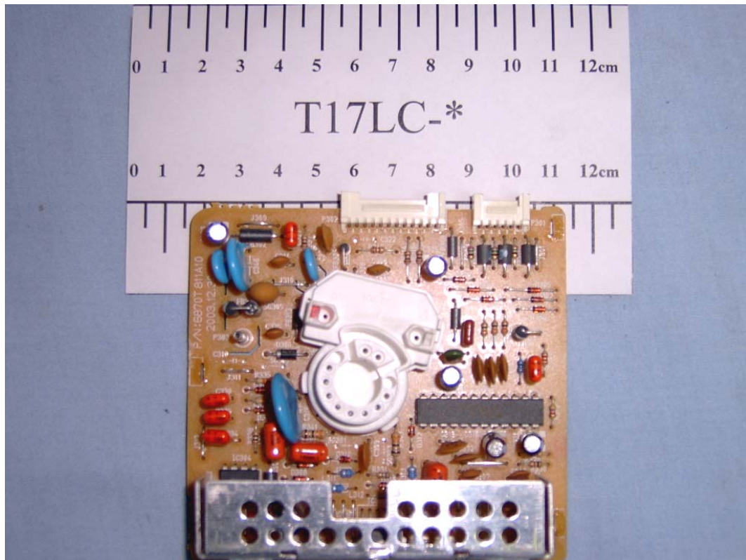
FIGURE 6 COLOR MONITOR (M/N:T17LC-*) CRT BOARD (COMPONENT SIDE)
