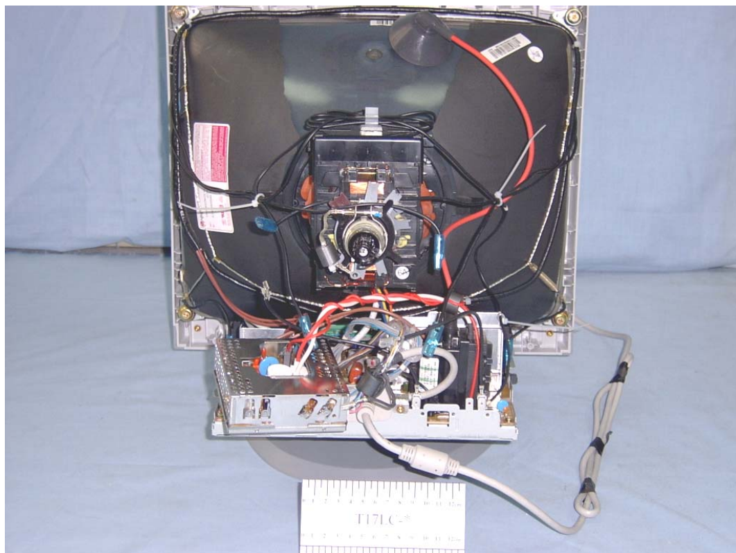
FIGURE 2 COLOR MONITOR (M/N:TI7LC-*) COVER REMOVED 2
