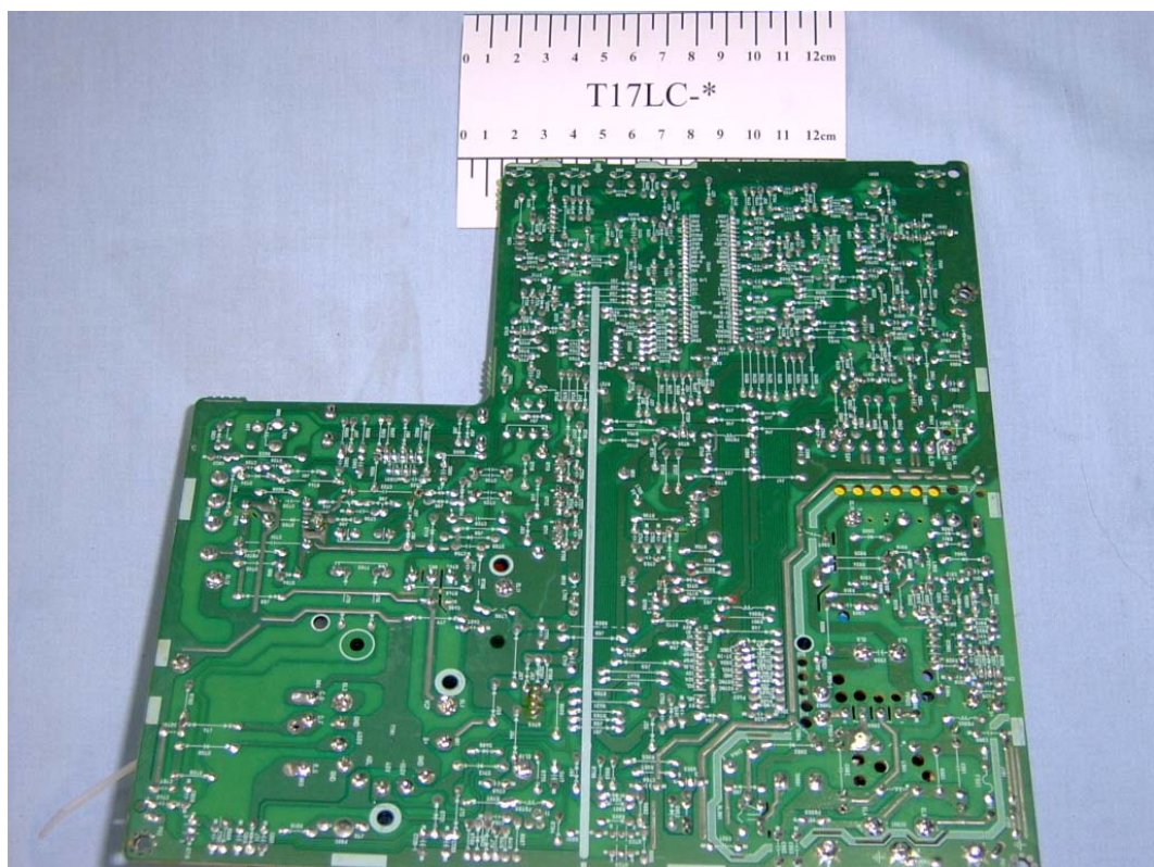
FIGURE 5 COLOR MONITOR (M/N:T17LC-*) MAIN BOARD (SOLDERED SIDE)
