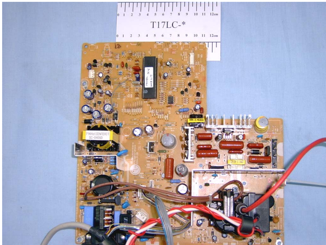
FIGURE 4 COLOR MONITOR (M/N:T17LC-*) MAIN BOARD (COMPONENT SIDE)
