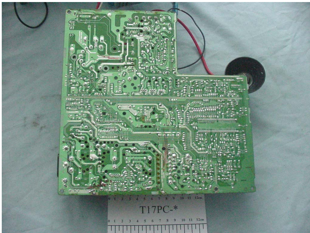
FIGURE 6 COLOR MONITOR (M/N: T17PC-*) MAIN BOARD (SOLDERED SIDE)
