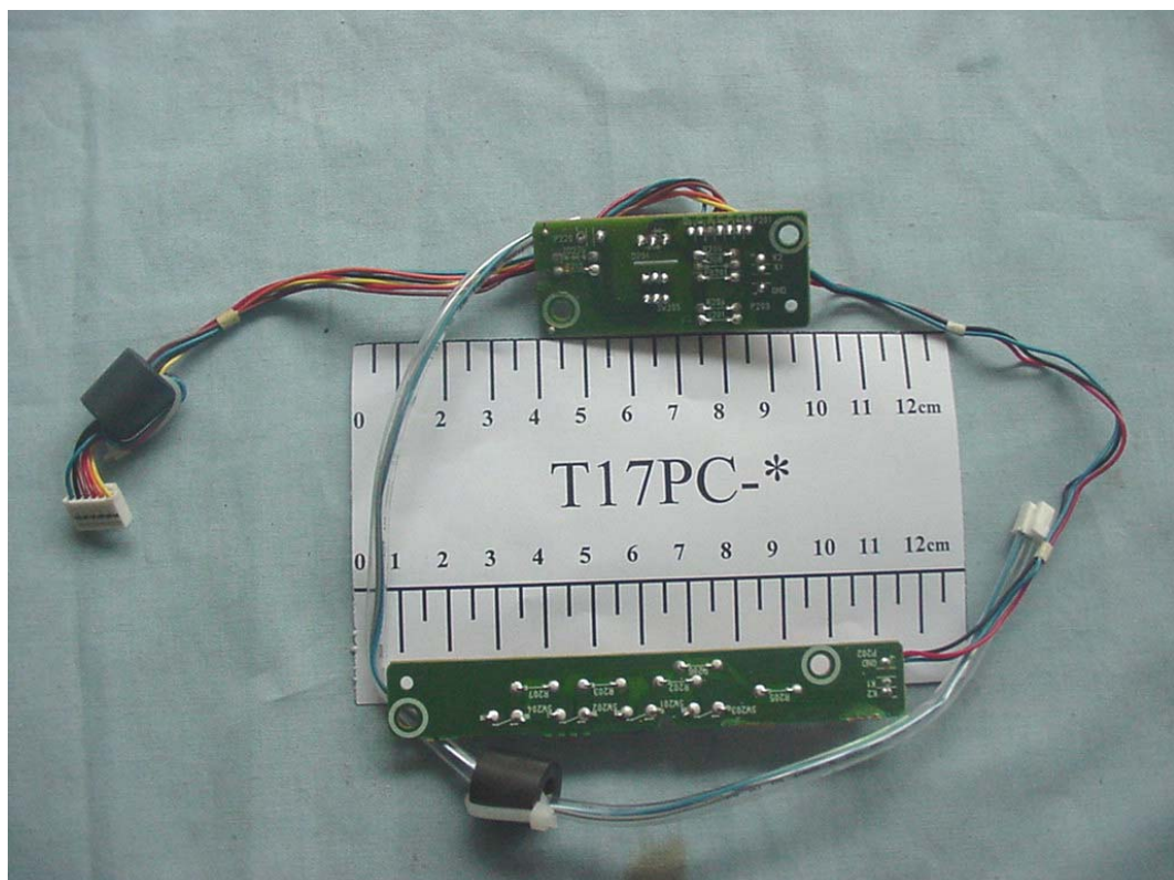
FIGURE 13 COLOR MONITOR (M/N: T17PC-*) BUTTON BOARD (SOLDERED SIDE)
