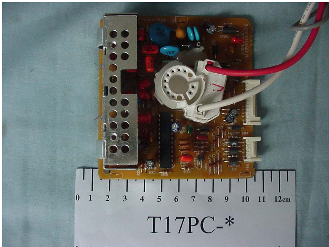
FIGURE 8 COLOR MONITOR (M/N: T17PC-*) CRT BOARD (COMPONENT SIDE)
