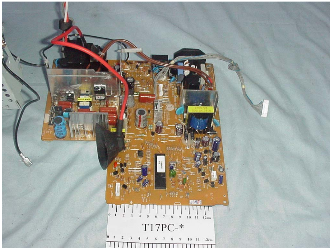
FIGURE 5 COLOR MONITOR (M/N: T17PC-*) MAIN BOARD (COMPONENT SIDE)
