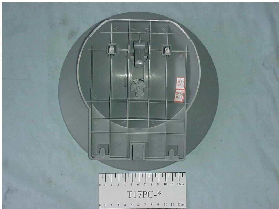
FIGURE 18 COLOR MONITOR (M/N: T17PC-*) BOTTOM HOLDER
