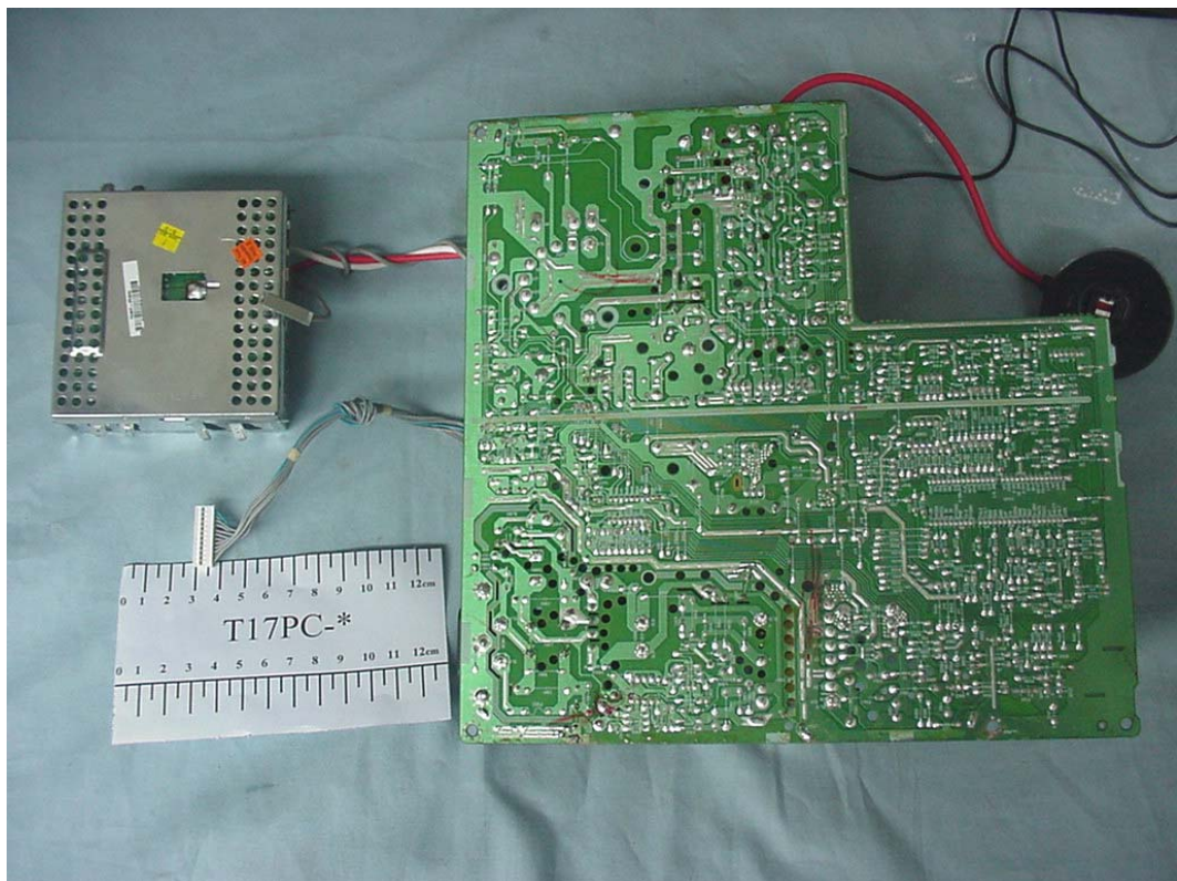
FIGURE 4 COLOR MONITOR (M/N: T17PC-*) MAIN BOARD & CRT BOARD (SOLDERED SIDE)
