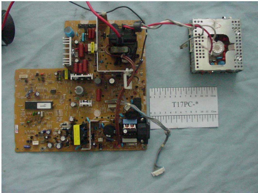
FIGURE 3 COLOR MONITOR (M/N: T17PC-*) MAIN BOARD & CRT BOARD (COMPONENT SIDE)
